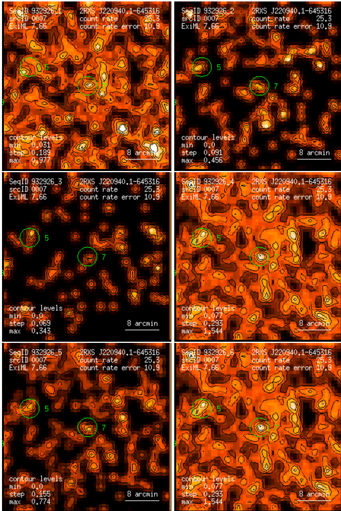
Figure 7: RASS 932926: detection 0007: band rate images, Gaussian filter: (1) PSPC channels 11 – 41, (2) 52 – 90, (3) 91 – 201, (4) 11 – 235, (5) 52 – 201, (6) 11 – 201. Broad band rates in counts/ks. Band rate contour levels in counts/ks/arcmin 2 .
