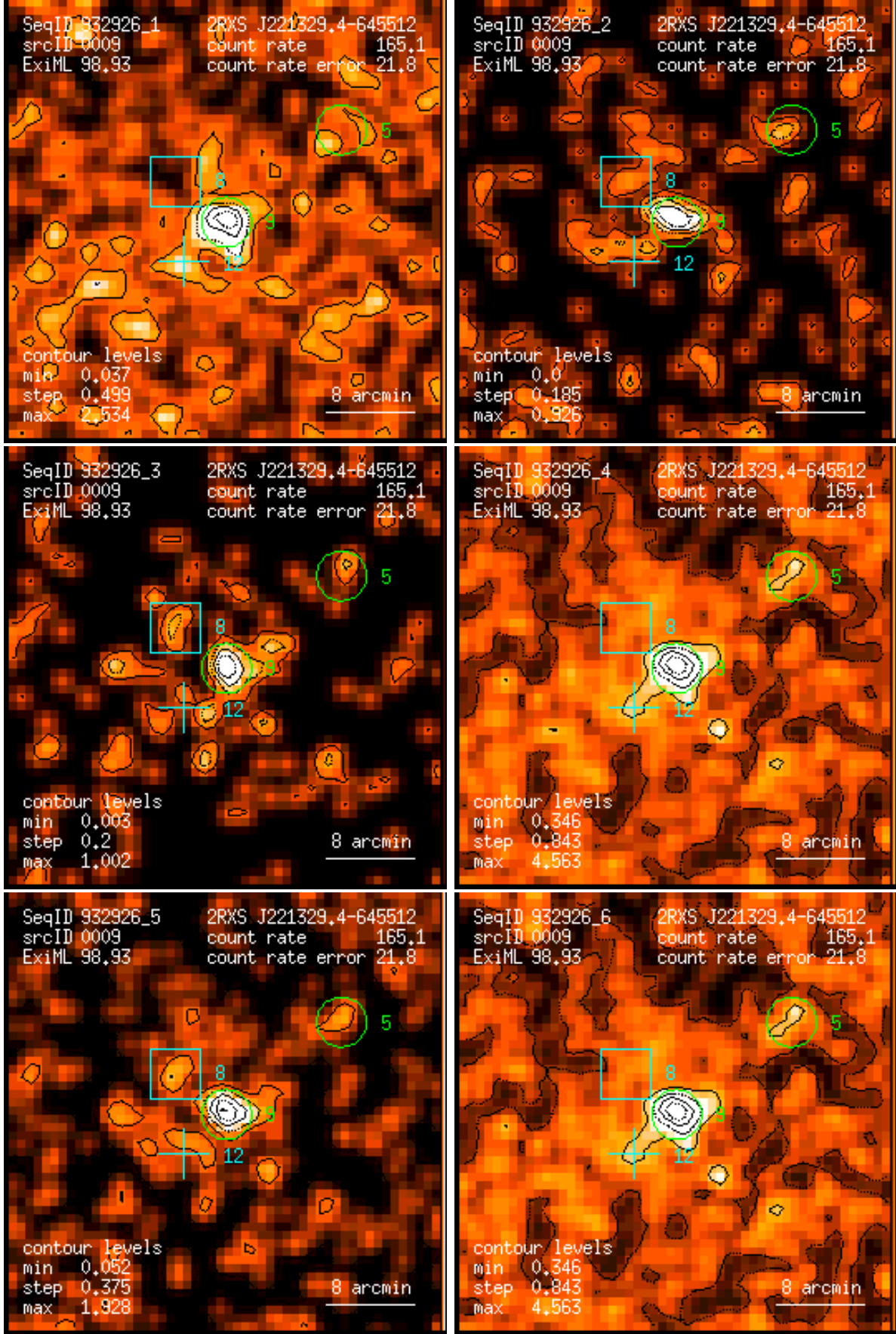
Figure 9: RASS 932926: detection 0009: band rate images, Gaussian filter: (1) PSPC channels 11 – 41, (2) 52 – 90, (3) 91 – 201, (4) 11 – 235, (5) 52 – 201, (6) 11 – 201. Broad band rates in counts/ks. Band rate contour levels in counts/ks/arcmin 2 .
