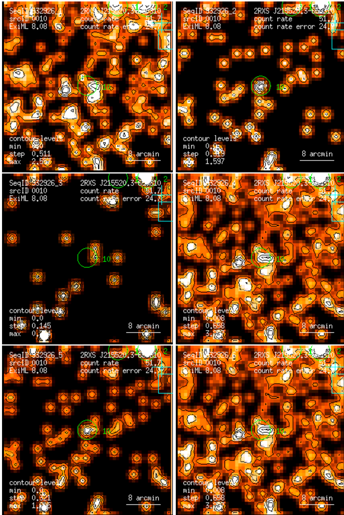
Figure 10: RASS 932926: detection 0010: band rate images, Gaussian filter: (1) PSPC channels 11 – 41, (2) 52 – 90, (3) 91 – 201, (4) 11 – 235, (5) 52 – 201, (6) 11 – 201. Broad band rates in counts/ks. Band rate contour levels in counts/ks/arcmin 2 .
