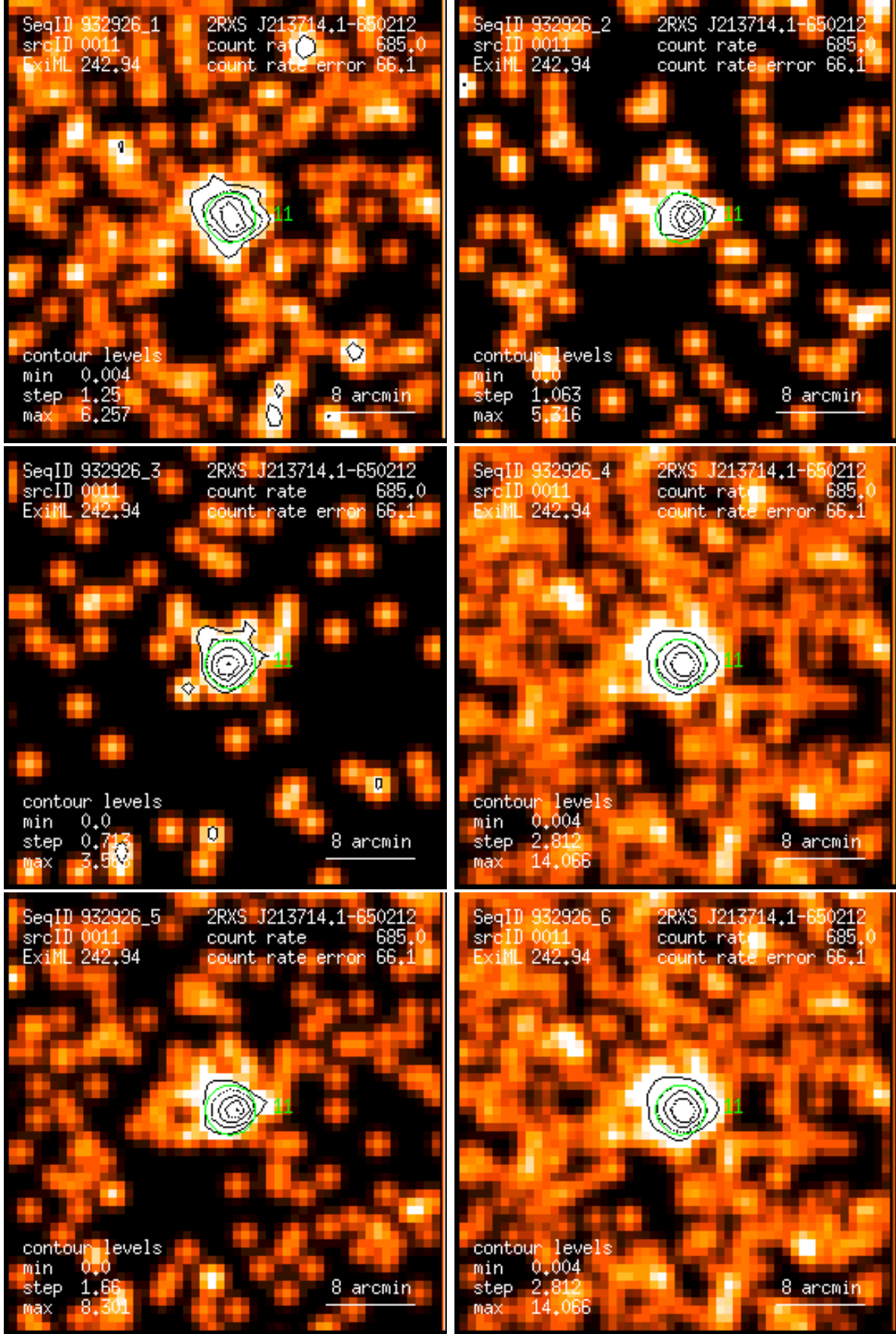
Figure 11: RASS 932926: detection 0011: band rate images, Gaussian filter: (1) PSPC channels 11 – 41, (2) 52 – 90, (3) 91 – 201, (4) 11 – 235, (5) 52 – 201, (6) 11 – 201. Broad band rates in counts/ks. Band rate contour levels in counts/ks/arcmin 2 .
