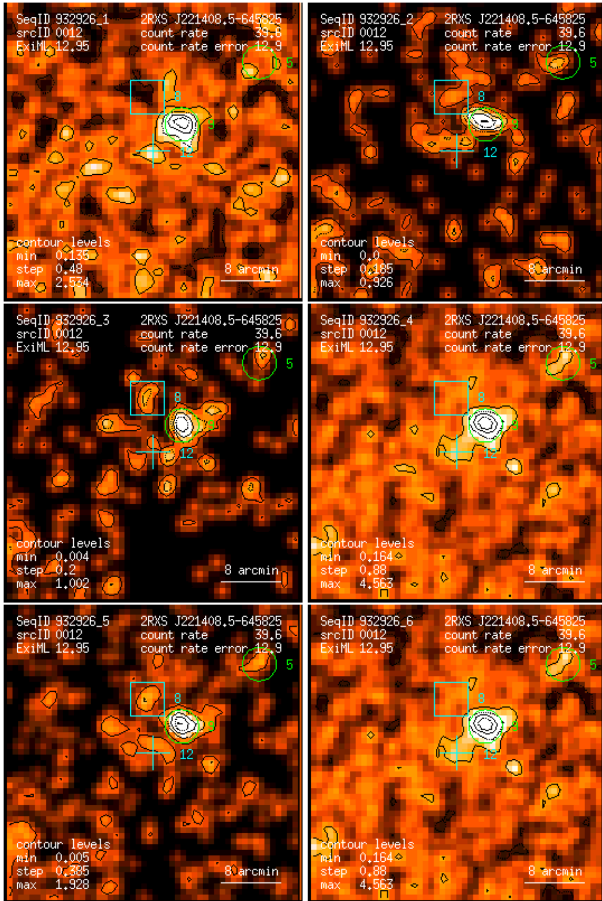
Figure 12: RASS 932926: detection 0012: band rate images, Gaussian filter: (1) PSPC channels 11 – 41, (2) 52 – 90, (3) 91 – 201, (4) 11 – 235, (5) 52 – 201, (6) 11 – 201. Broad band rates in counts/ks. Band rate contour levels in counts/ks/arcmin 2 .
