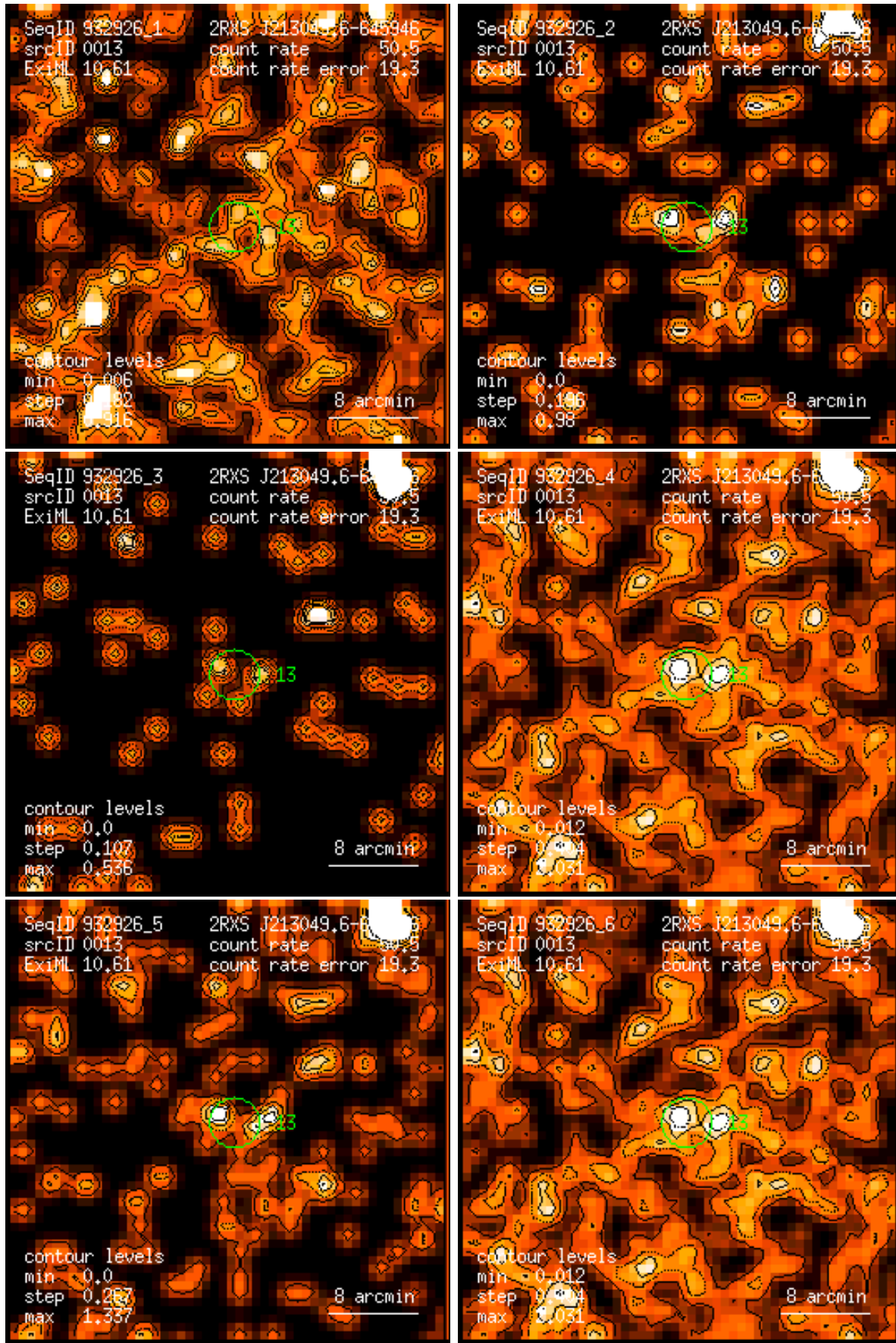
Figure 13: RASS 932926: detection 0013: band rate images, Gaussian filter: (1) PSPC channels 11 – 41, (2) 52 – 90, (3) 91 – 201, (4) 11 – 235, (5) 52 – 201, (6) 11 – 201. Broad band rates in counts/ks. Band rate contour levels in counts/ks/arcmin 2 .
