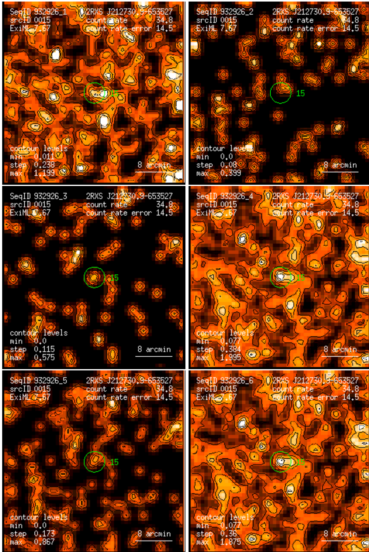
Figure 15: RASS 932926: detection 0015: band rate images, Gaussian filter: (1) PSPC channels 11 – 41, (2) 52 – 90, (3) 91 – 201, (4) 11 – 235, (5) 52 – 201, (6) 11 – 201. Broad band rates in counts/ks. Band rate contour levels in counts/ks/arcmin 2 .
