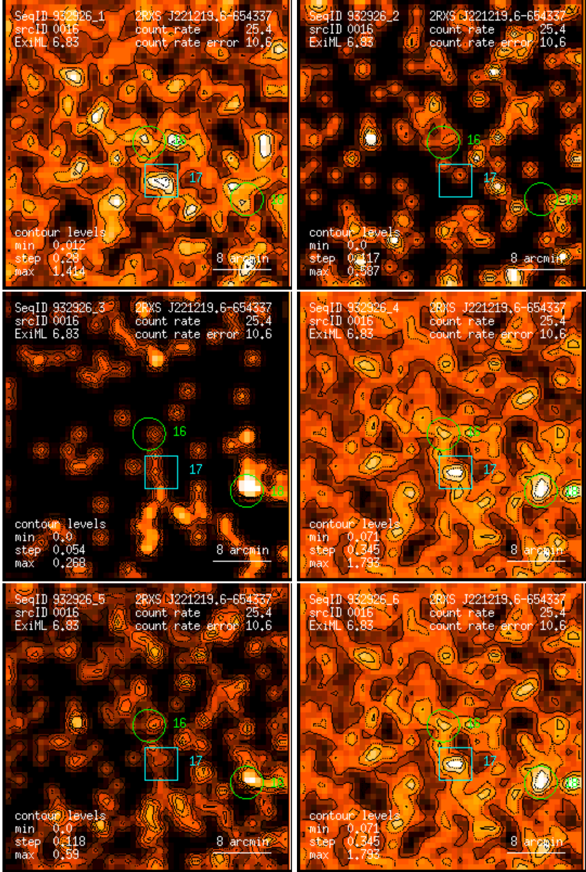
Figure 16: RASS 932926: detection 0016: band rate images, Gaussian filter: (1) PSPC channels 11 – 41, (2) 52 – 90, (3) 91 – 201, (4) 11 – 235, (5) 52 – 201, (6) 11 – 201. Broad band rates in counts/ks. Band rate contour levels in counts/ks/arcmin 2 .
