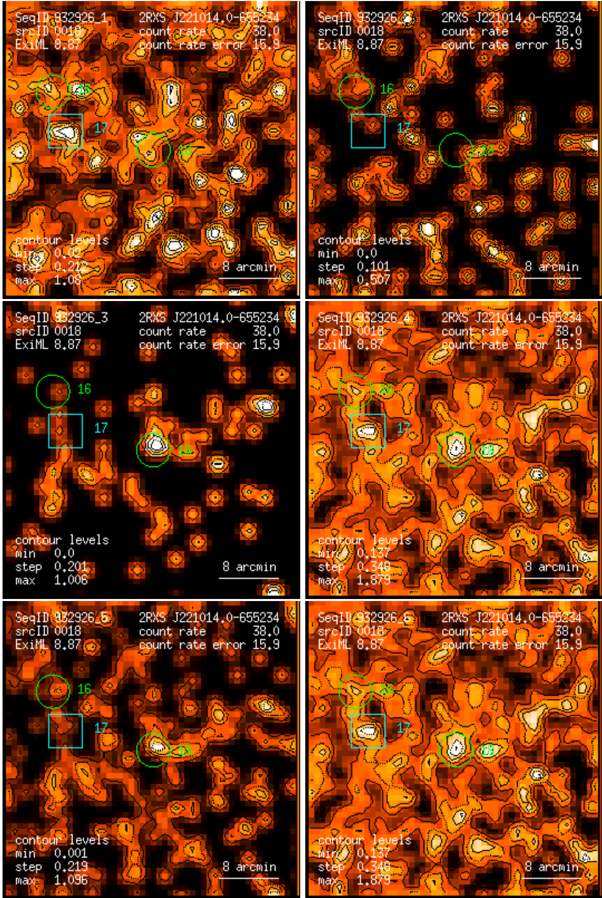
Figure 18: RASS 932926: detection 0018: band rate images, Gaussian filter: (1) PSPC channels 11 – 41, (2) 52 – 90, (3) 91 – 201, (4) 11 – 235, (5) 52 – 201, (6) 11 – 201. Broad band rates in counts/ks. Band rate contour levels in counts/ks/arcmin 2 .
