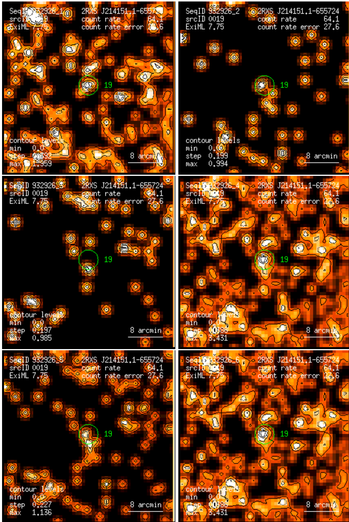
Figure 19: RASS 932926: detection 0019: band rate images, Gaussian filter: (1) PSPC channels 11 – 41, (2) 52 – 90, (3) 91 – 201, (4) 11 – 235, (5) 52 – 201, (6) 11 – 201. Broad band rates in counts/ks. Band rate contour levels in counts/ks/arcmin 2 .
