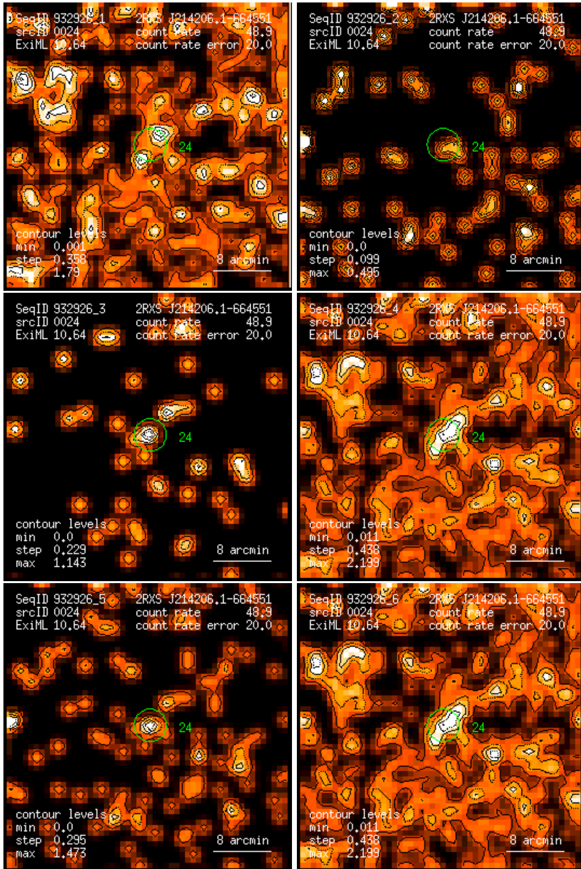
Figure 24: RASS 932926: detection 0024: band rate images, Gaussian filter: (1) PSPC channels 11 – 41, (2) 52 – 90, (3) 91 – 201, (4) 11 – 235, (5) 52 – 201, (6) 11 – 201. Broad band rates in counts/ks. Band rate contour levels in counts/ks/arcmin 2 .
