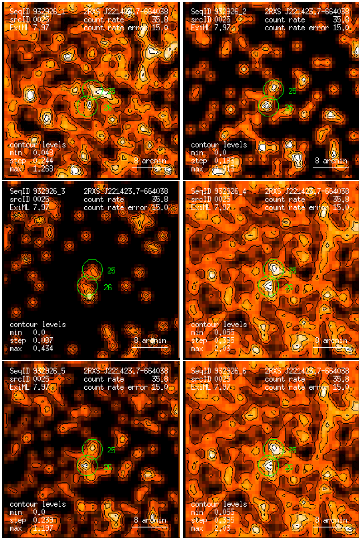
Figure 25: RASS 932926: detection 0025: band rate images, Gaussian filter: (1) PSPC channels 11 – 41, (2) 52 – 90, (3) 91 – 201, (4) 11 – 235, (5) 52 – 201, (6) 11 – 201. Broad band rates in counts/ks. Band rate contour levels in counts/ks/arcmin 2 .
