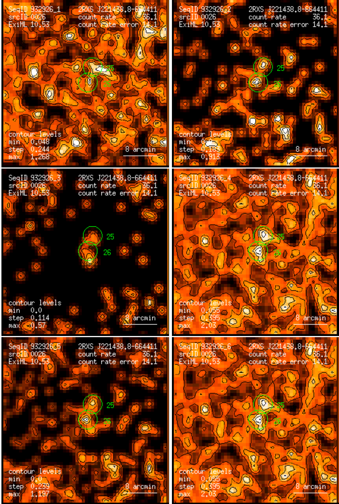
Figure 26: RASS 932926: detection 0026: band rate images, Gaussian filter: (1) PSPC channels 11 – 41, (2) 52 – 90, (3) 91 – 201, (4) 11 – 235, (5) 52 – 201, (6) 11 – 201. Broad band rates in counts/ks. Band rate contour levels in counts/ks/arcmin 2 .
