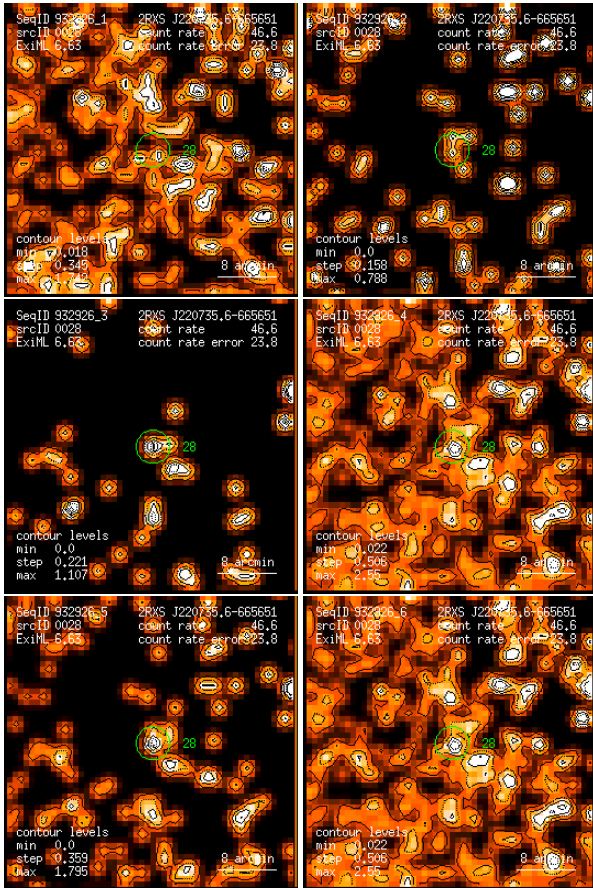
Figure 28: RASS 932926: detection 0028: band rate images, Gaussian filter: (1) PSPC channels 11 – 41, (2) 52 – 90, (3) 91 – 201, (4) 11 – 235, (5) 52 – 201, (6) 11 – 201. Broad band rates in counts/ks. Band rate contour levels in counts/ks/arcmin 2 .
