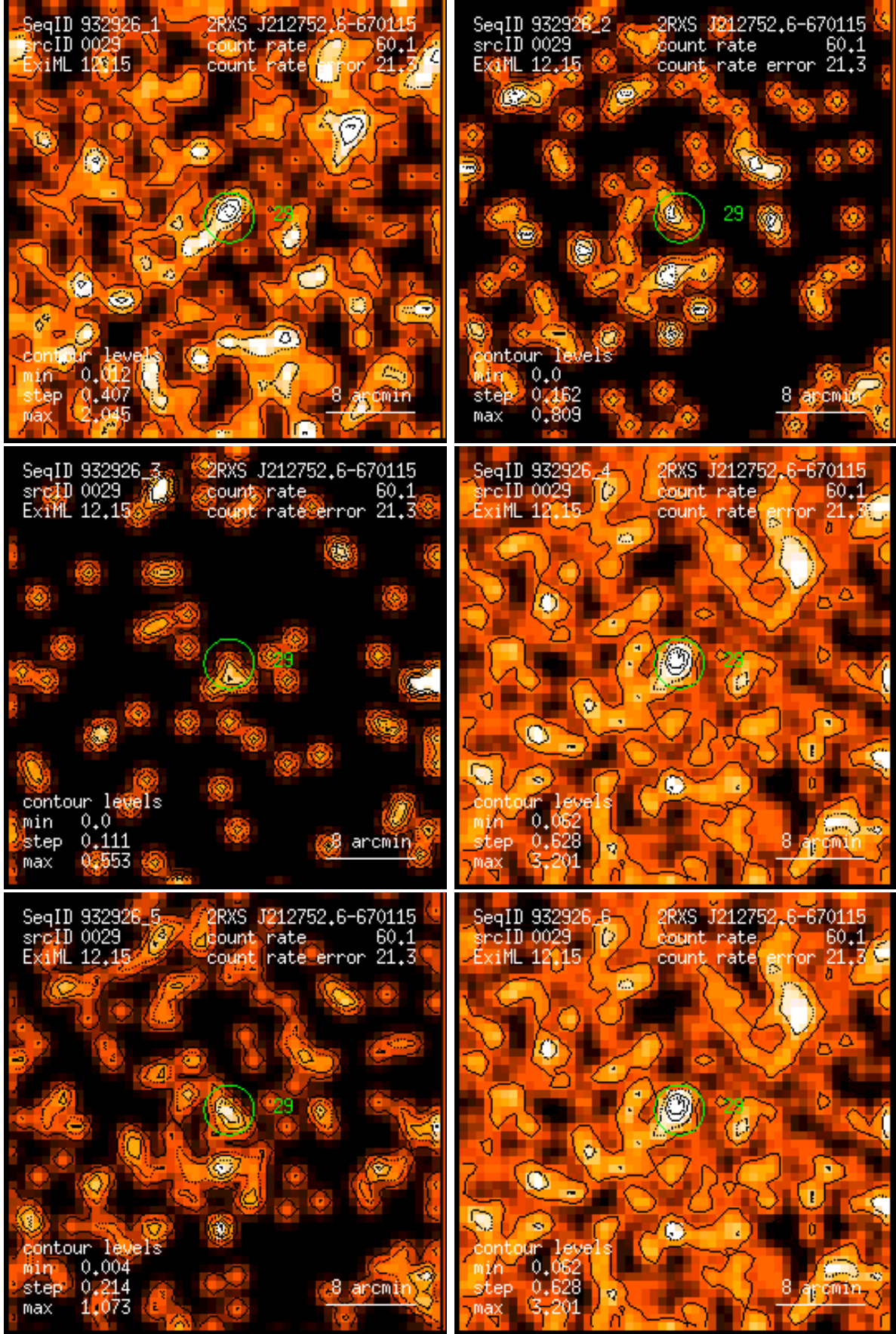
Figure 29: RASS 932926: detection 0029: band rate images, Gaussian filter: (1) PSPC channels 11 – 41, (2) 52 – 90, (3) 91 – 201, (4) 11 – 235, (5) 52 – 201, (6) 11 – 201. Broad band rates in counts/ks. Band rate contour levels in counts/ks/arcmin 2 .
