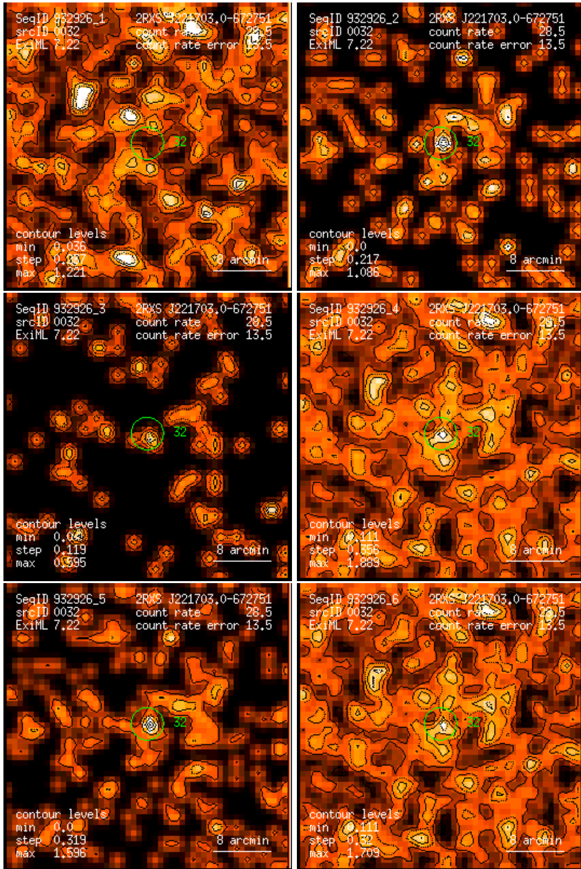
Figure 32: RASS 932926: detection 0032: band rate images, Gaussian filter: (1) PSPC channels 11 – 41, (2) 52 – 90, (3) 91 – 201, (4) 11 – 235, (5) 52 – 201, (6) 11 – 201. Broad band rates in counts/ks. Band rate contour levels in counts/ks/arcmin 2 .
