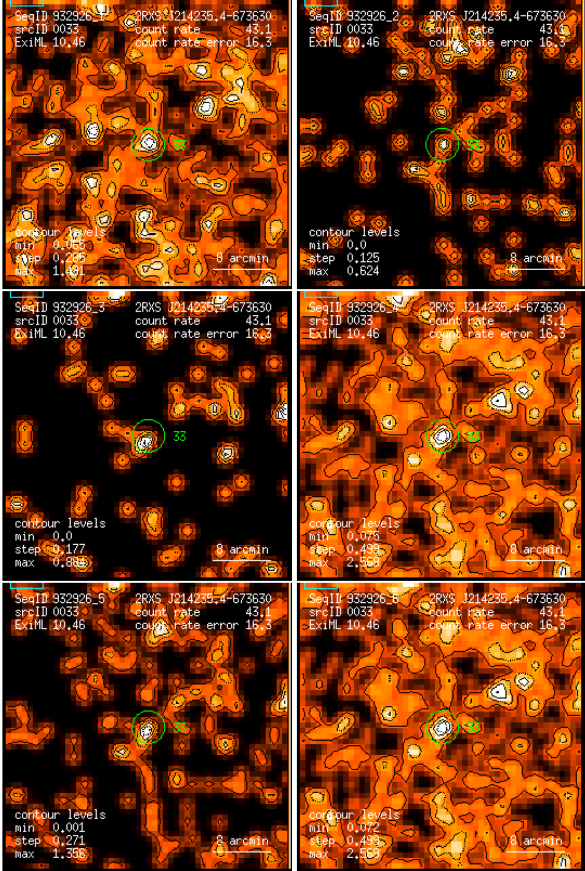
Figure 33: RASS 932926: detection 0033: band rate images, Gaussian filter: (1) PSPC channels 11 – 41, (2) 52 – 90, (3) 91 – 201, (4) 11 – 235, (5) 52 – 201, (6) 11 – 201. Broad band rates in counts/ks. Band rate contour levels in counts/ks/arcmin 2 .
