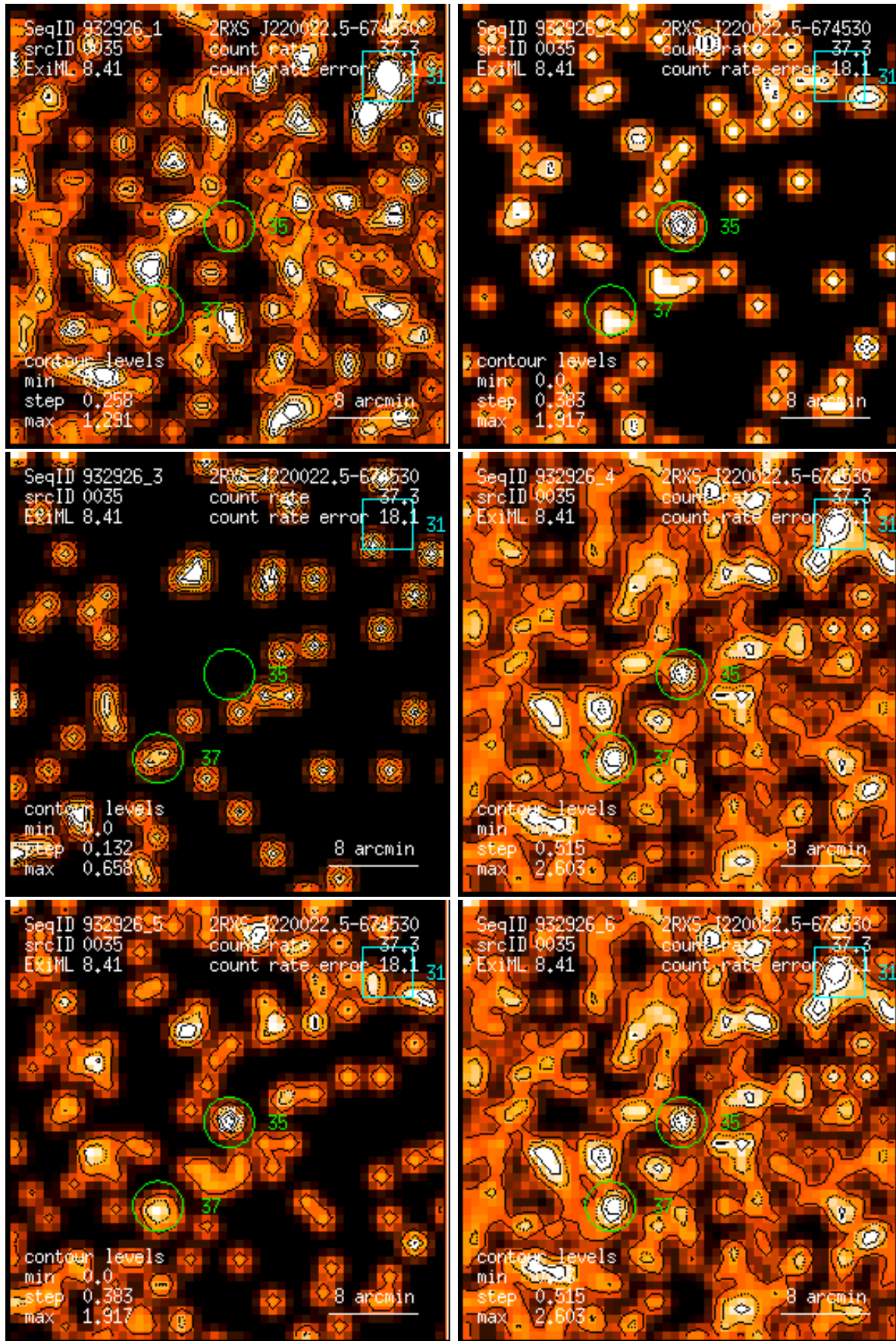
Figure 35: RASS 932926: detection 0035: band rate images, Gaussian filter: (1) PSPC channels 11 – 41, (2) 52 – 90, (3) 91 – 201, (4) 11 – 235, (5) 52 – 201, (6) 11 – 201. Broad band rates in counts/ks. Band rate contour levels in counts/ks/arcmin 2 .
