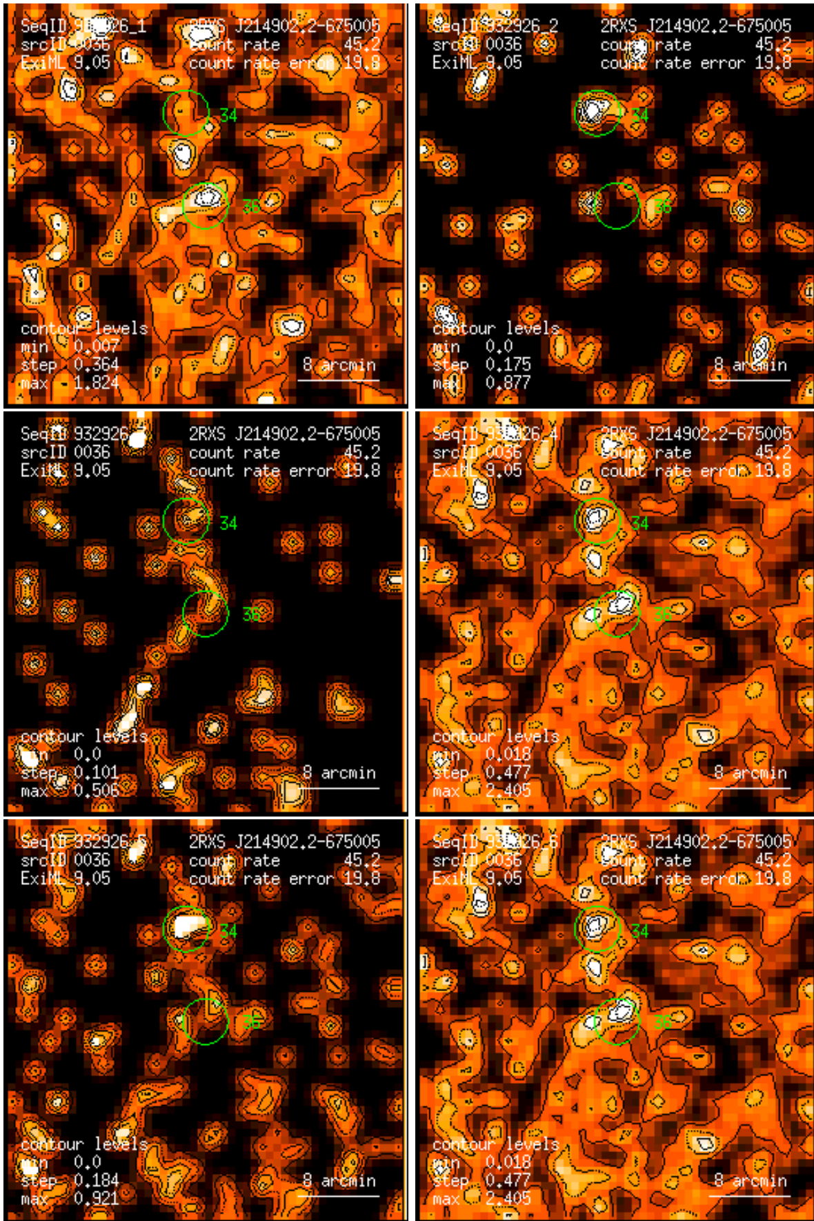
Figure 36: RASS 932926: detection 0036: band rate images, Gaussian filter: (1) PSPC channels 11 – 41, (2) 52 – 90, (3) 91 – 201, (4) 11 – 235, (5) 52 – 201, (6) 11 – 201. Broad band rates in counts/ks. Band rate contour levels in counts/ks/arcmin 2 .
