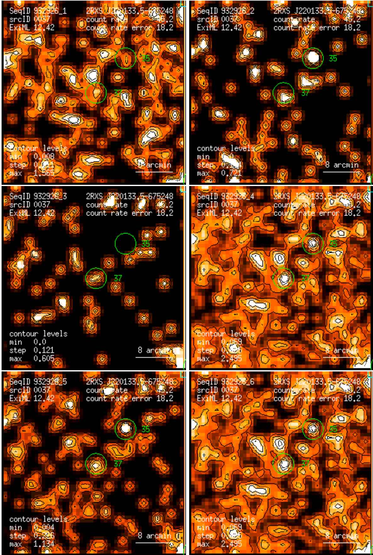
Figure 37: RASS 932926: detection 0037: band rate images, Gaussian filter: (1) PSPC channels 11 – 41, (2) 52 – 90, (3) 91 – 201, (4) 11 – 235, (5) 52 – 201, (6) 11 – 201. Broad band rates in counts/ks. Band rate contour levels in counts/ks/arcmin 2 .
