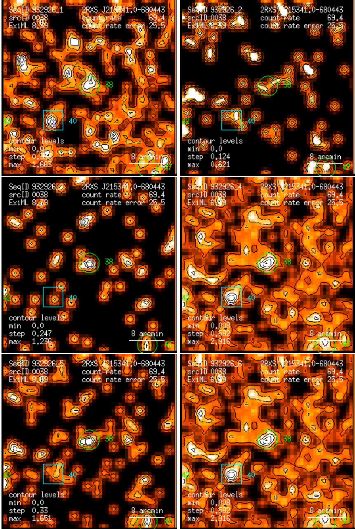
Figure 38: RASS 932926: detection 0038: band rate images, Gaussian filter: (1) PSPC channels 11 – 41, (2) 52 – 90, (3) 91 – 201, (4) 11 – 235, (5) 52 – 201, (6) 11 – 201. Broad band rates in counts/ks. Band rate contour levels in counts/ks/arcmin 2 .
