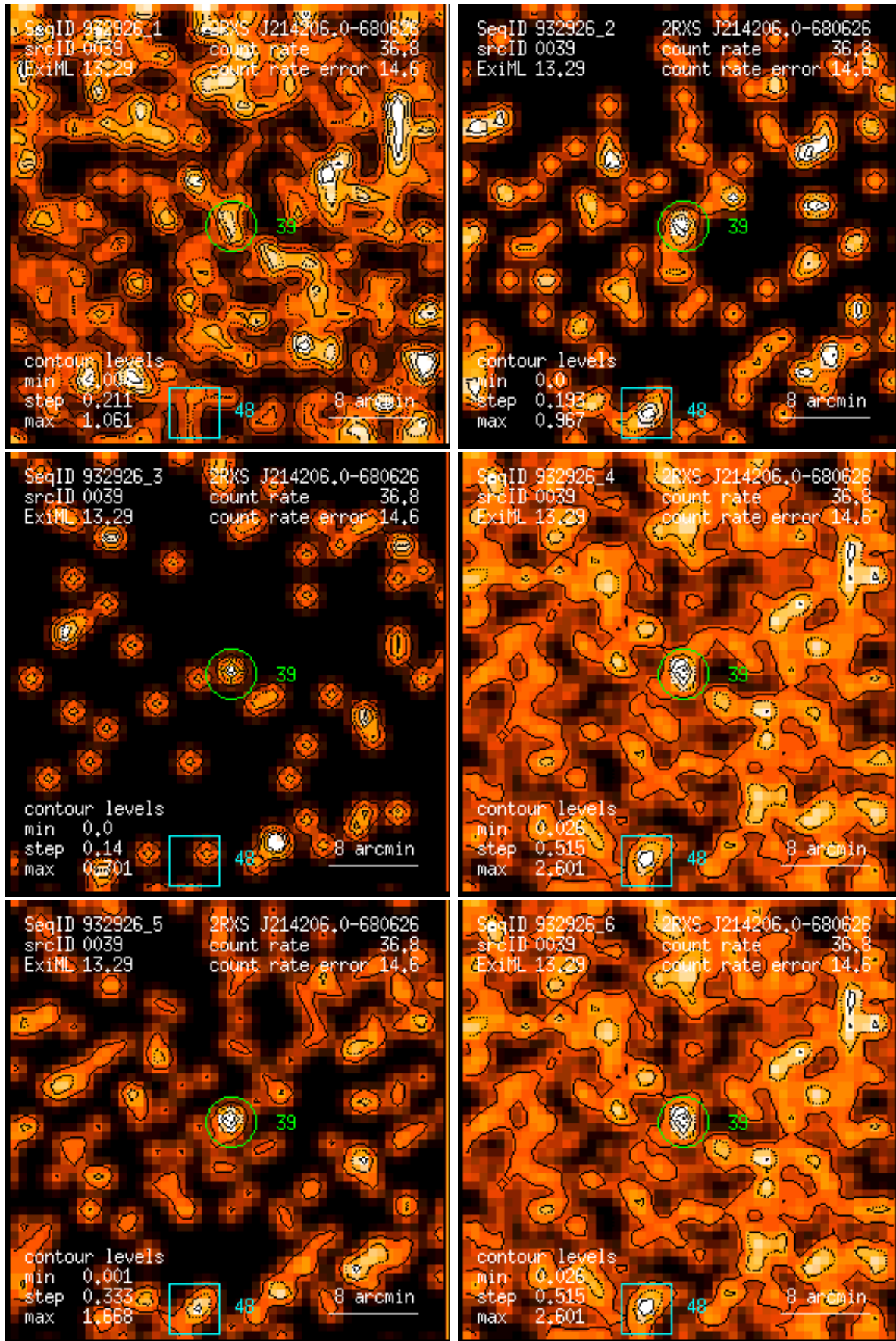
Figure 39: RASS 932926: detection 0039: band rate images, Gaussian filter: (1) PSPC channels 11 – 41, (2) 52 – 90, (3) 91 – 201, (4) 11 – 235, (5) 52 – 201, (6) 11 – 201. Broad band rates in counts/ks. Band rate contour levels in counts/ks/arcmin 2 .
