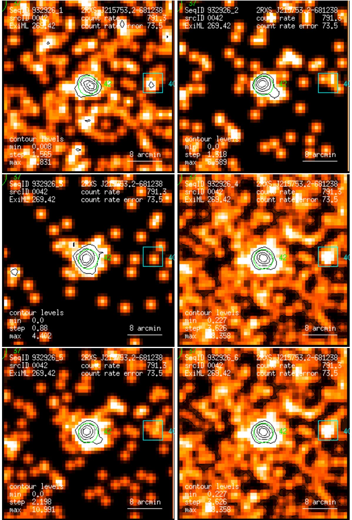
Figure 42: RASS 932926: detection 0042: band rate images, Gaussian filter: (1) PSPC channels 11 – 41, (2) 52 – 90, (3) 91 – 201, (4) 11 – 235, (5) 52 – 201, (6) 11 – 201. Broad band rates in counts/ks. Band rate contour levels in counts/ks/arcmin 2 .
