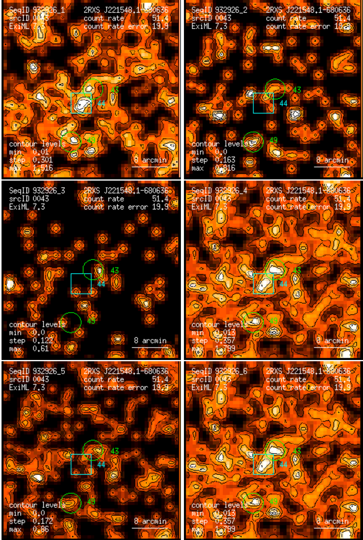
Figure 43: RASS 932926: detection 0043: band rate images, Gaussian filter: (1) PSPC channels 11 – 41, (2) 52 – 90, (3) 91 – 201, (4) 11 – 235, (5) 52 – 201, (6) 11 – 201. Broad band rates in counts/ks. Band rate contour levels in counts/ks/arcmin 2 .
