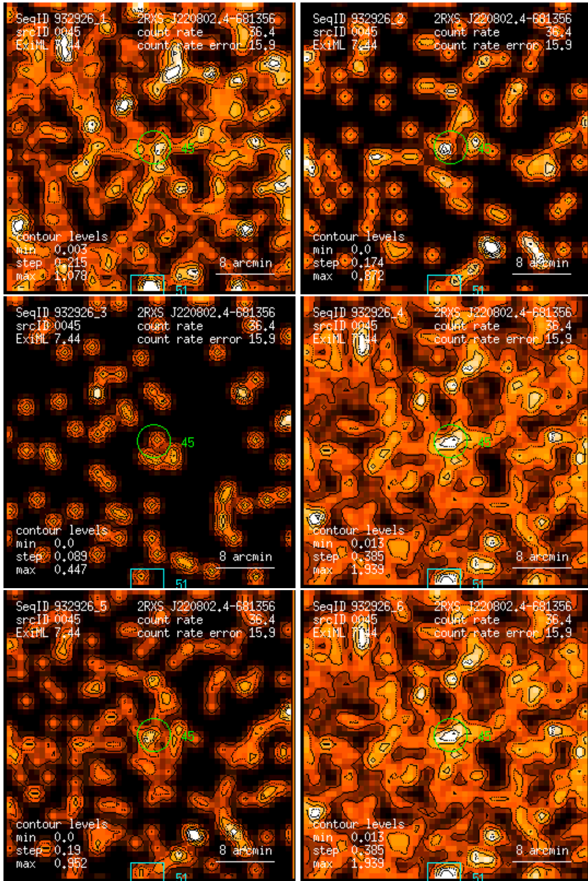
Figure 45: RASS 932926: detection 0045: band rate images, Gaussian filter: (1) PSPC channels 11 – 41, (2) 52 – 90, (3) 91 – 201, (4) 11 – 235, (5) 52 – 201, (6) 11 – 201. Broad band rates in counts/ks. Band rate contour levels in counts/ks/arcmin 2 .
