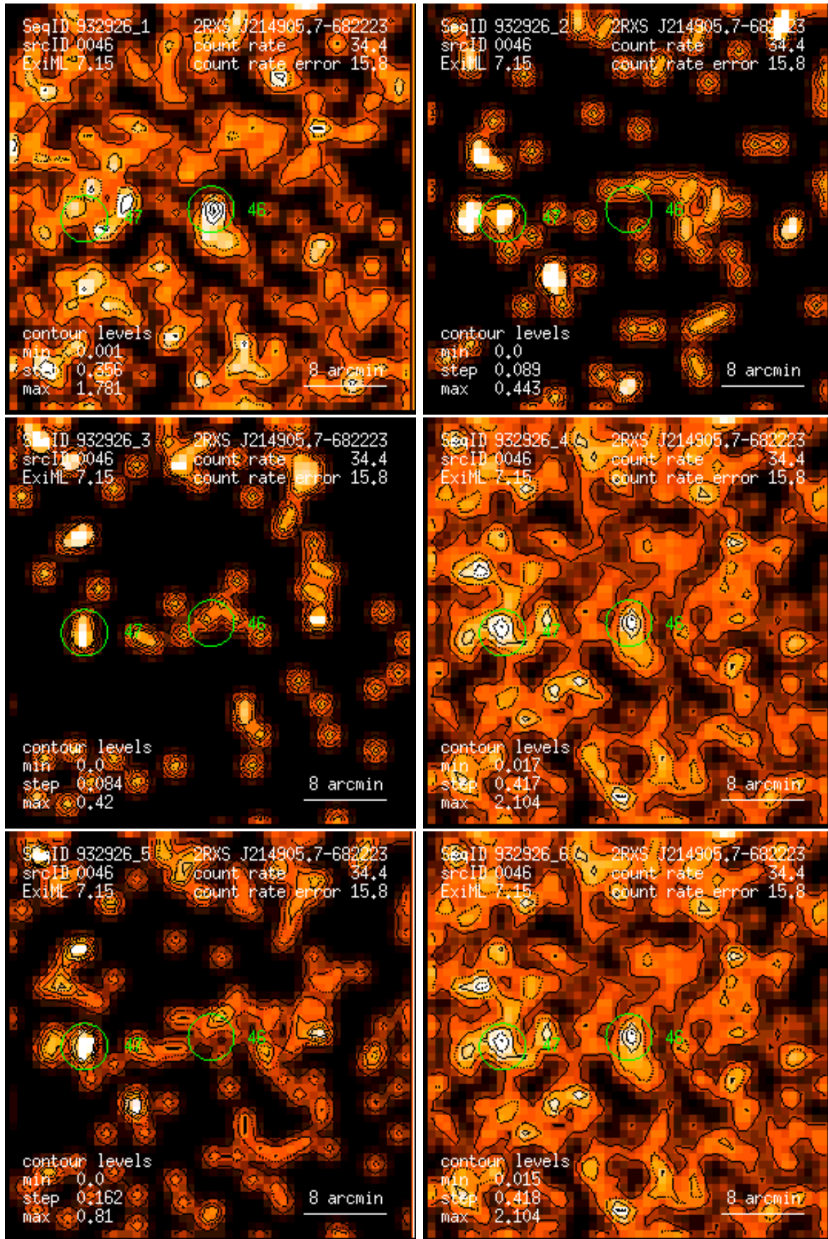
Figure 46: RASS 932926: detection 0046: band rate images, Gaussian filter: (1) PSPC channels 11 – 41, (2) 52 – 90, (3) 91 – 201, (4) 11 – 235, (5) 52 – 201, (6) 11 – 201. Broad band rates in counts/ks. Band rate contour levels in counts/ks/arcmin 2 .
