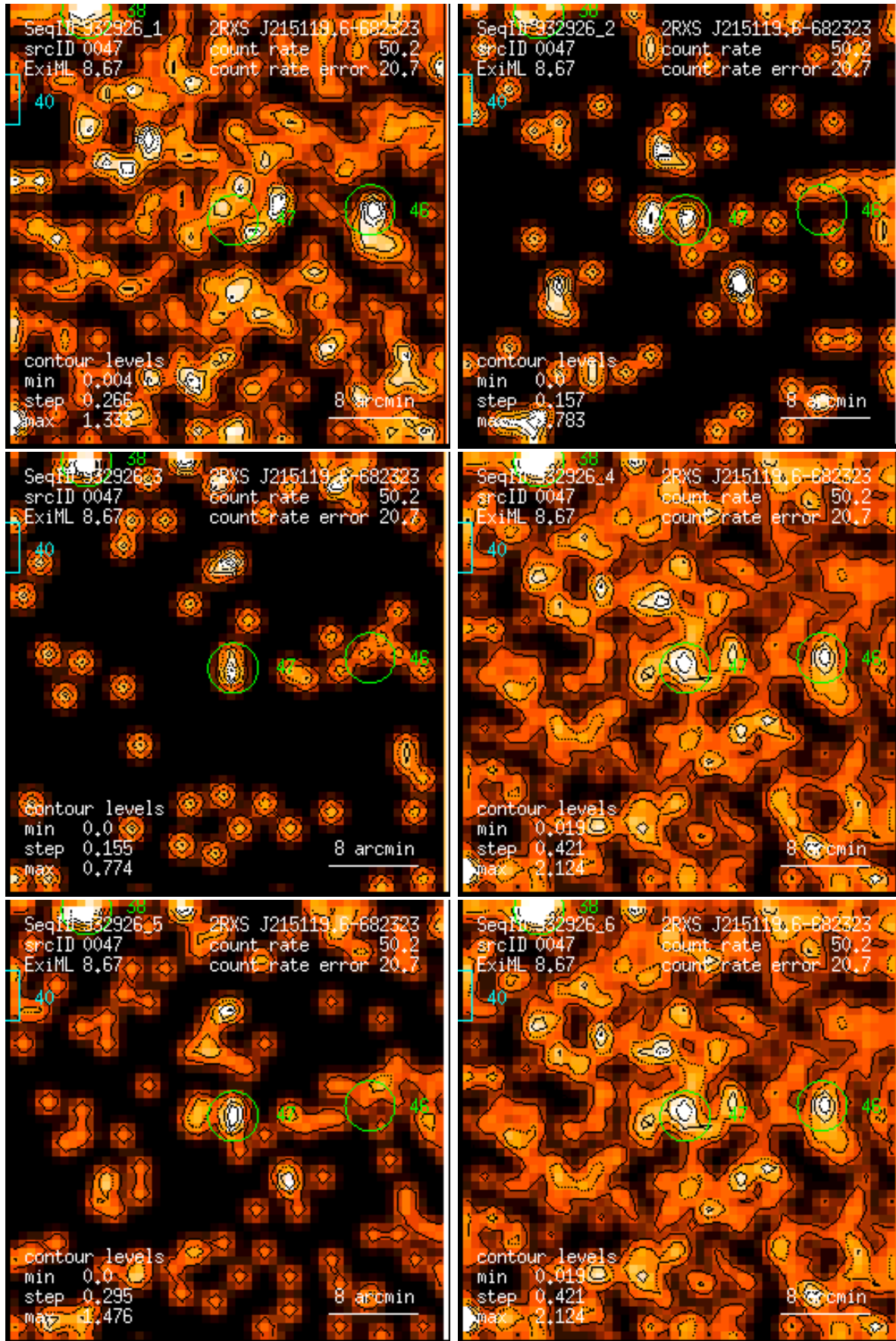
Figure 47: RASS 932926: detection 0047: band rate images, Gaussian filter: (1) PSPC channels 11 – 41, (2) 52 – 90, (3) 91 – 201, (4) 11 – 235, (5) 52 – 201, (6) 11 – 201. Broad band rates in counts/ks. Band rate contour levels in counts/ks/arcmin 2 .
