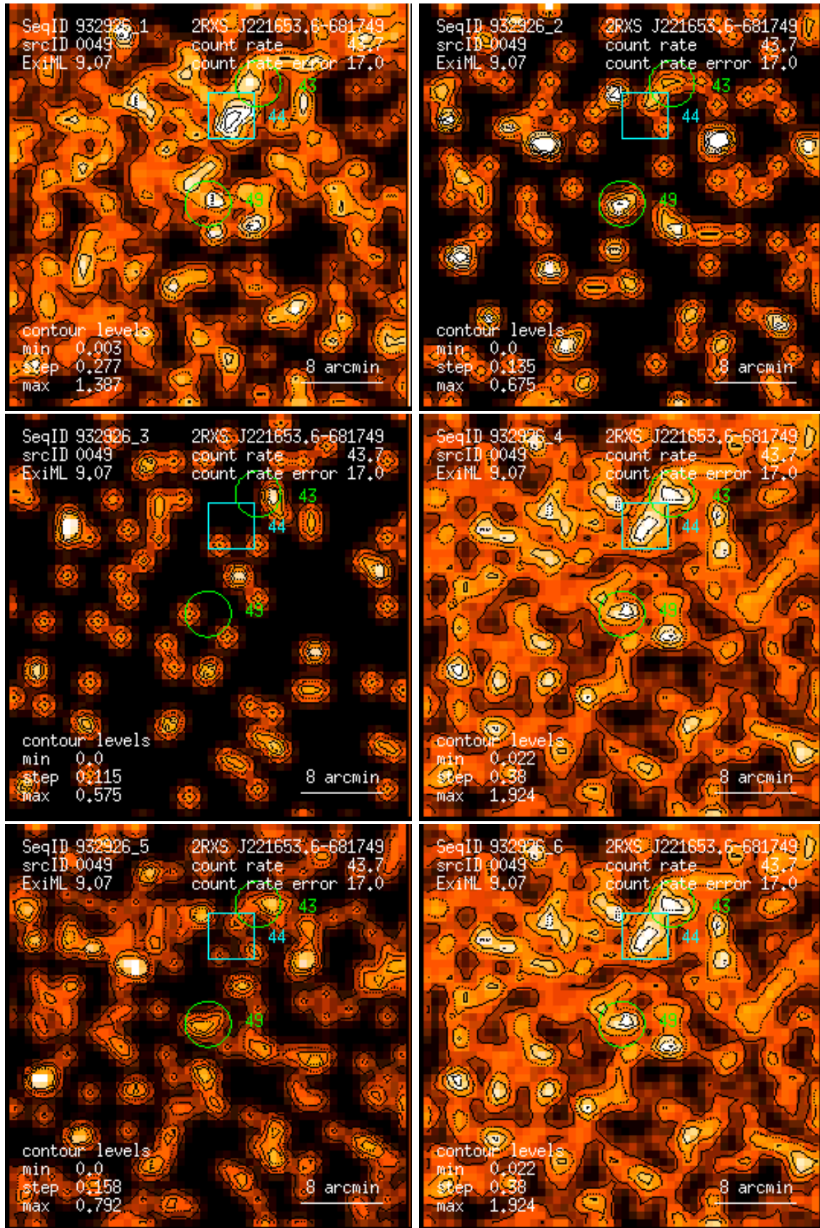
Figure 49: RASS 932926: detection 0049: band rate images, Gaussian filter: (1) PSPC channels 11 – 41, (2) 52 – 90, (3) 91 – 201, (4) 11 – 235, (5) 52 – 201, (6) 11 – 201. Broad band rates in counts/ks. Band rate contour levels in counts/ks/arcmin 2 .
