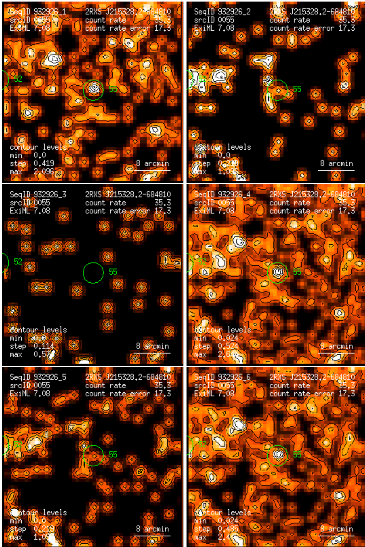
Figure 55: RASS 932926: detection 0055: band rate images, Gaussian filter: (1) PSPC channels 11 – 41, (2) 52 – 90, (3) 91 – 201, (4) 11 – 235, (5) 52 – 201, (6) 11 – 201. Broad band rates in counts/ks. Band rate contour levels in counts/ks/arcmin 2 .
