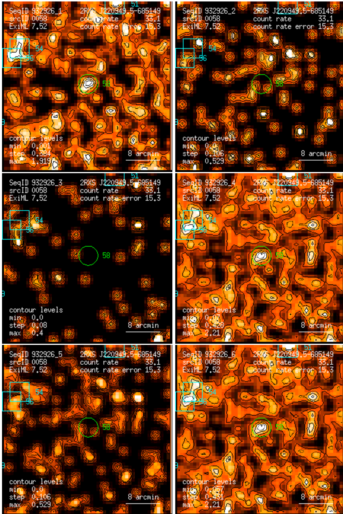
Figure 58: RASS 932926: detection 0058: band rate images, Gaussian filter: (1) PSPC channels 11 – 41, (2) 52 – 90, (3) 91 – 201, (4) 11 – 235, (5) 52 – 201, (6) 11 – 201. Broad band rates in counts/ks. Band rate contour levels in counts/ks/arcmin 2 .
