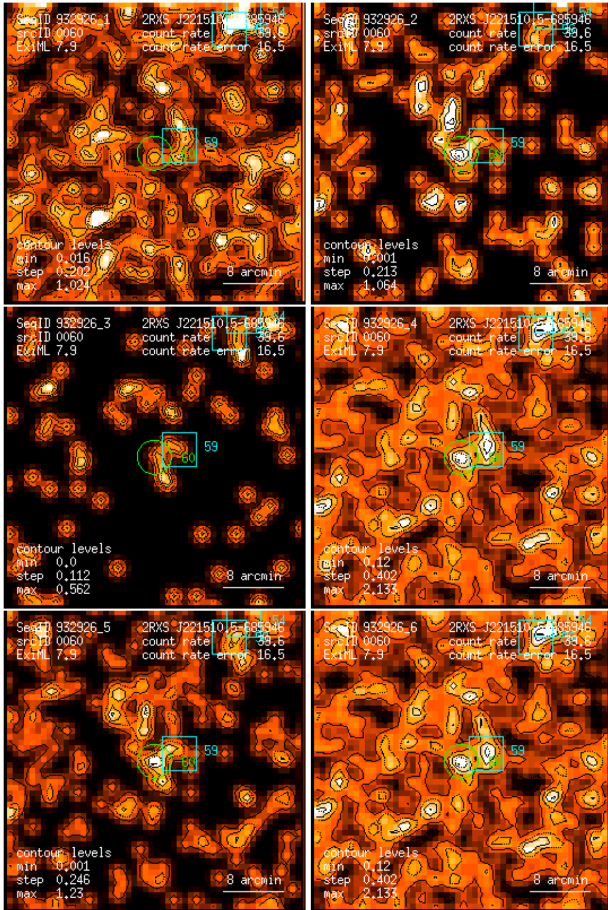
Figure 60: RASS 932926: detection 0060: band rate images, Gaussian filter: (1) PSPC channels 11 – 41, (2) 52 – 90, (3) 91 – 201, (4) 11 – 235, (5) 52 – 201, (6) 11 – 201. Broad band rates in counts/ks. Band rate contour levels in counts/ks/arcmin 2 .
