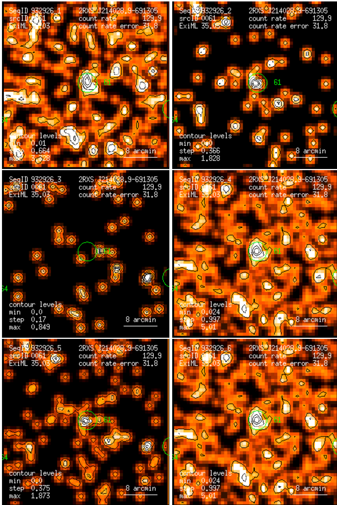
Figure 61: RASS 932926: detection 0061: band rate images, Gaussian filter: (1) PSPC channels 11 – 41, (2) 52 – 90, (3) 91 – 201, (4) 11 – 235, (5) 52 – 201, (6) 11 – 201. Broad band rates in counts/ks. Band rate contour levels in counts/ks/arcmin 2 .
