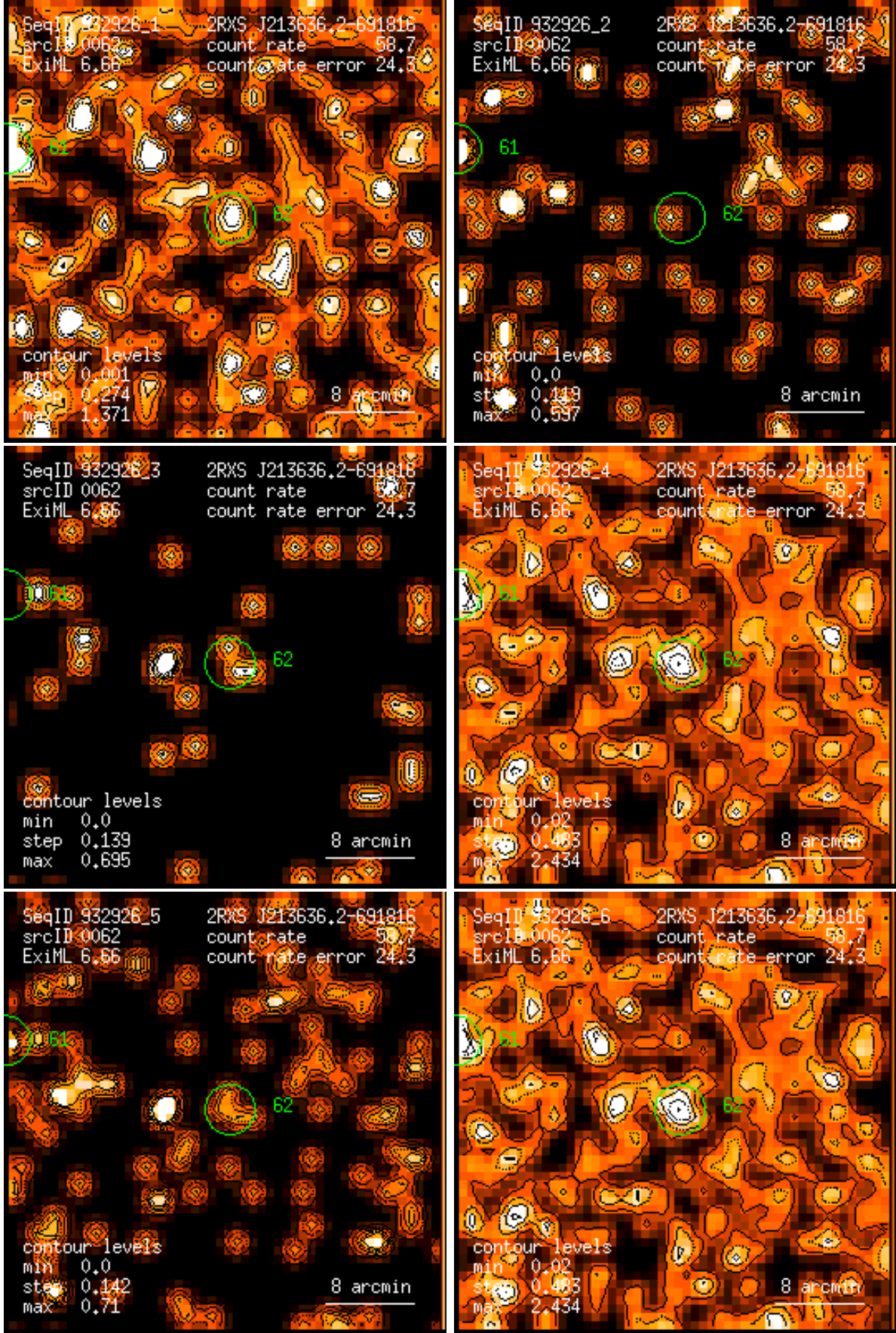
Figure 62: RASS 932926: detection 0062: band rate images, Gaussian filter: (1) PSPC channels 11 – 41, (2) 52 – 90, (3) 91 – 201, (4) 11 – 235, (5) 52 – 201, (6) 11 – 201. Broad band rates in counts/ks. Band rate contour levels in counts/ks/arcmin 2 .
