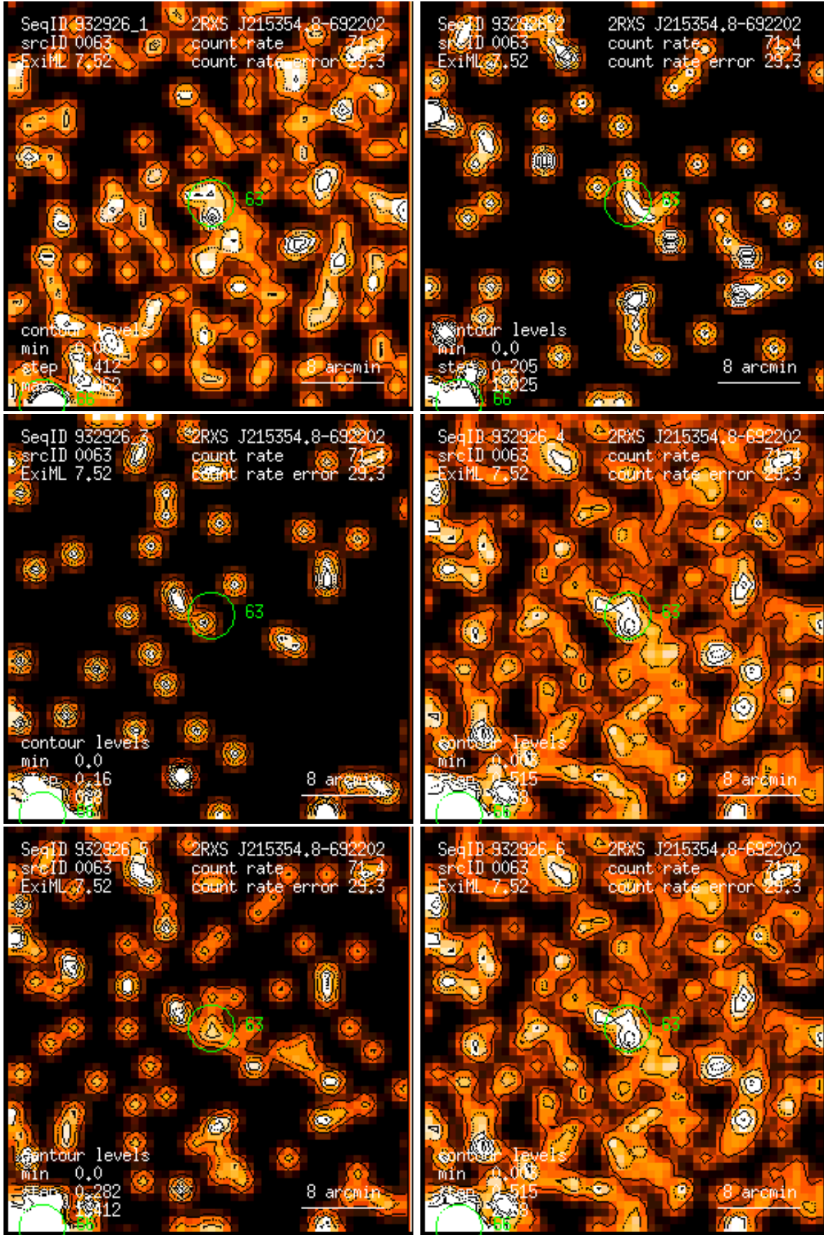
Figure 63: RASS 932926: detection 0063: band rate images, Gaussian filter: (1) PSPC channels 11 – 41, (2) 52 – 90, (3) 91 – 201, (4) 11 – 235, (5) 52 – 201, (6) 11 – 201. Broad band rates in counts/ks. Band rate contour levels in counts/ks/arcmin 2 .
