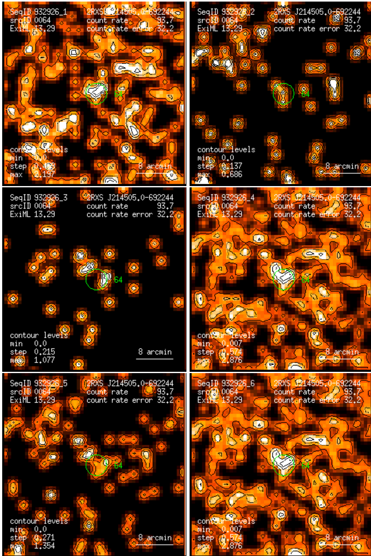
Figure 64: RASS 932926: detection 0064: band rate images, Gaussian filter: (1) PSPC channels 11 – 41, (2) 52 – 90, (3) 91 – 201, (4) 11 – 235, (5) 52 – 201, (6) 11 – 201. Broad band rates in counts/ks. Band rate contour levels in counts/ks/arcmin 2 .
