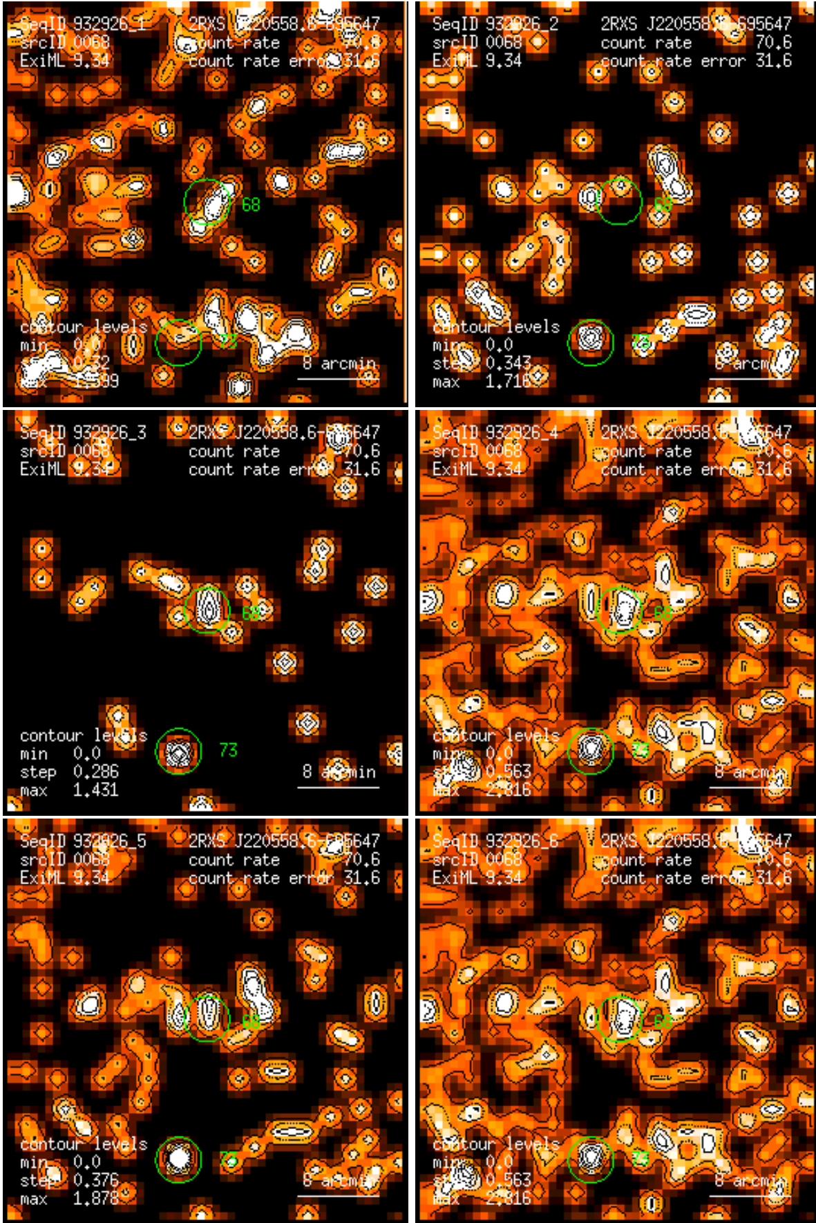
Figure 68: RASS 932926: detection 0068: band rate images, Gaussian filter: (1) PSPC channels 11 – 41, (2) 52 – 90, (3) 91 – 201, (4) 11 – 235, (5) 52 – 201, (6) 11 – 201. Broad band rates in counts/ks. Band rate contour levels in counts/ks/arcmin 2 .
