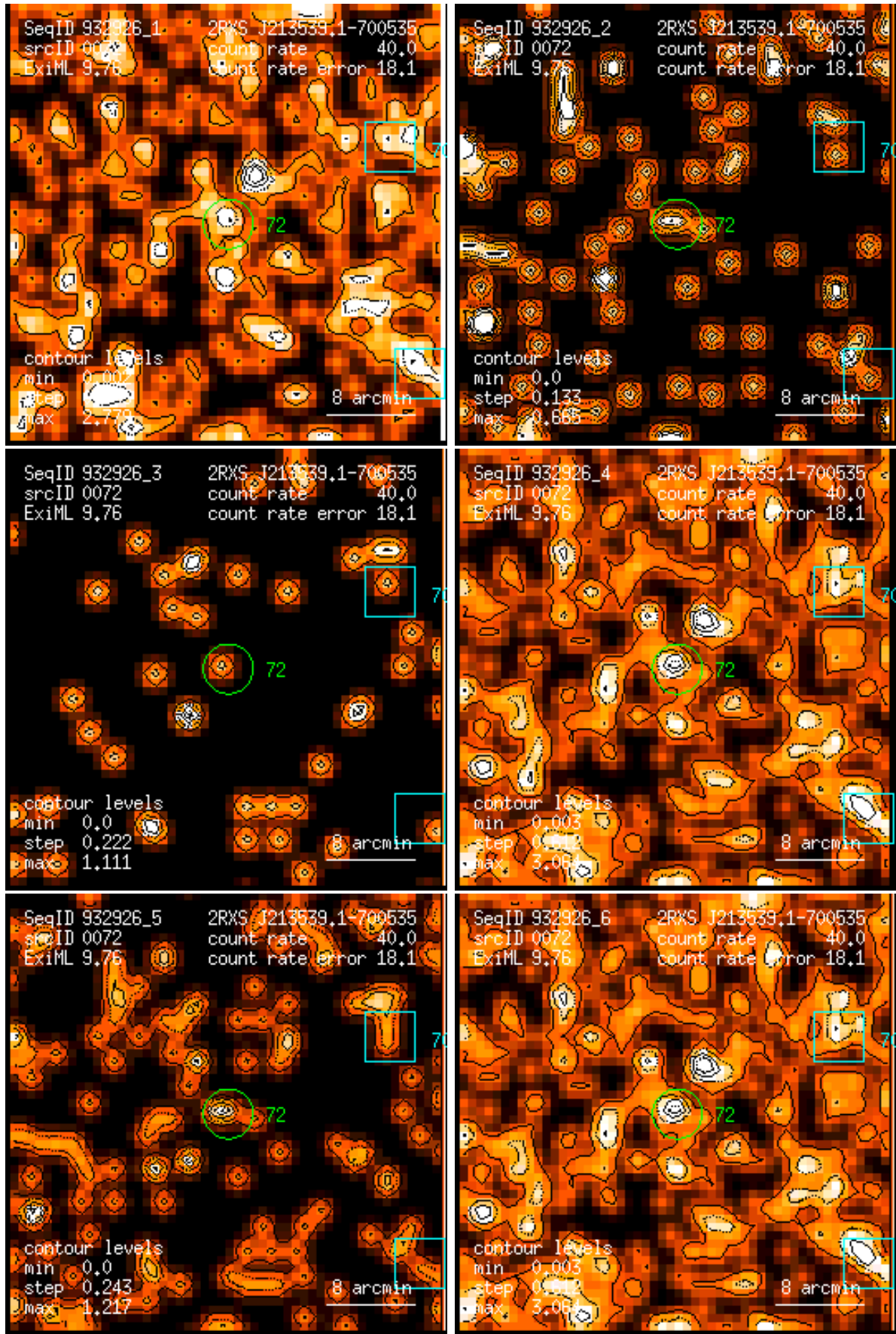
Figure 72: RASS 932926: detection 0072: band rate images, Gaussian filter: (1) PSPC channels 11 – 41, (2) 52 – 90, (3) 91 – 201, (4) 11 – 235, (5) 52 – 201, (6) 11 – 201. Broad band rates in counts/ks. Band rate contour levels in counts/ks/arcmin 2 .
