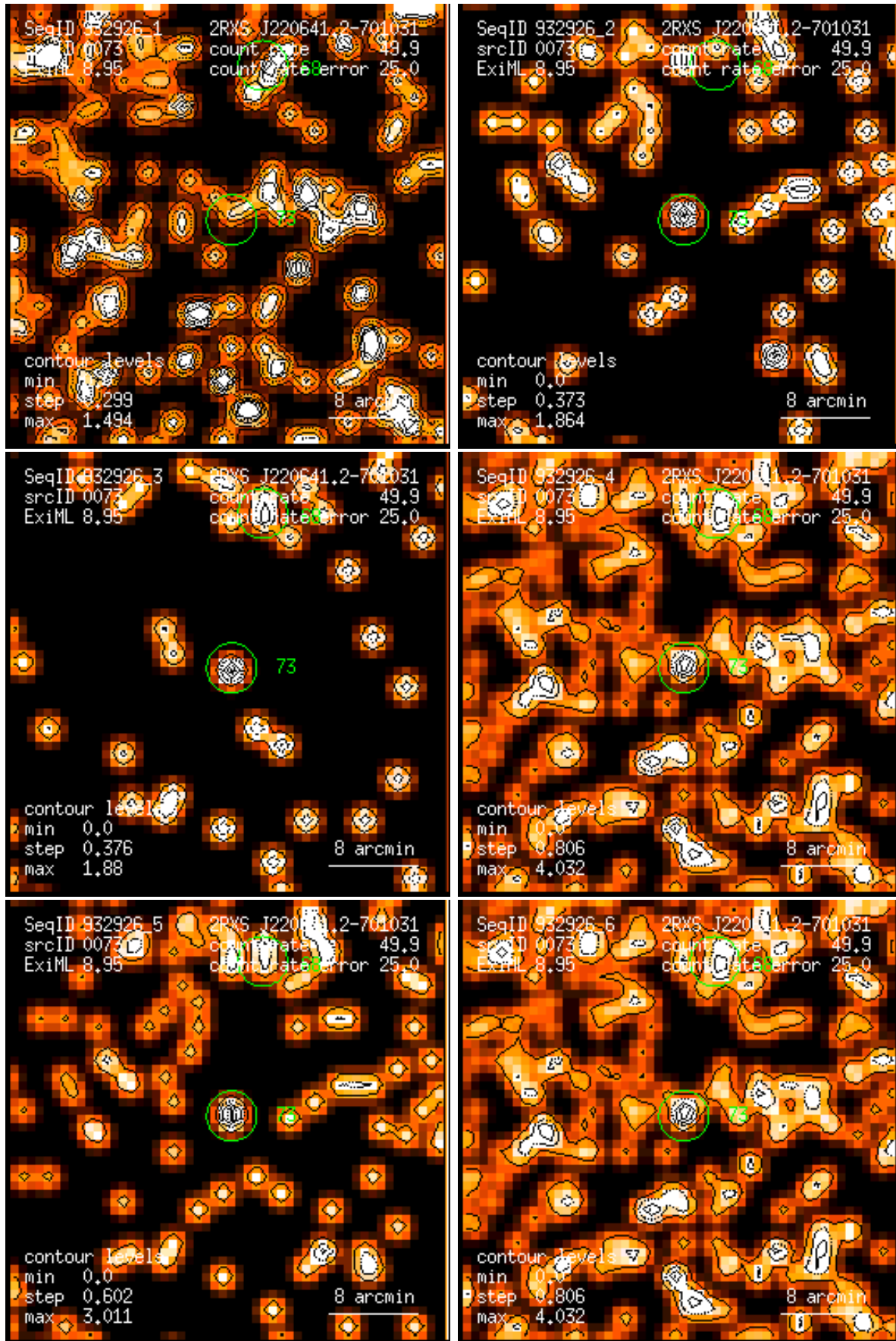
Figure 73: RASS 932926: detection 0073: band rate images, Gaussian filter: (1) PSPC channels 11 – 41, (2) 52 – 90, (3) 91 – 201, (4) 11 – 235, (5) 52 – 201, (6) 11 – 201. Broad band rates in counts/ks. Band rate contour levels in counts/ks/arcmin 2 .
