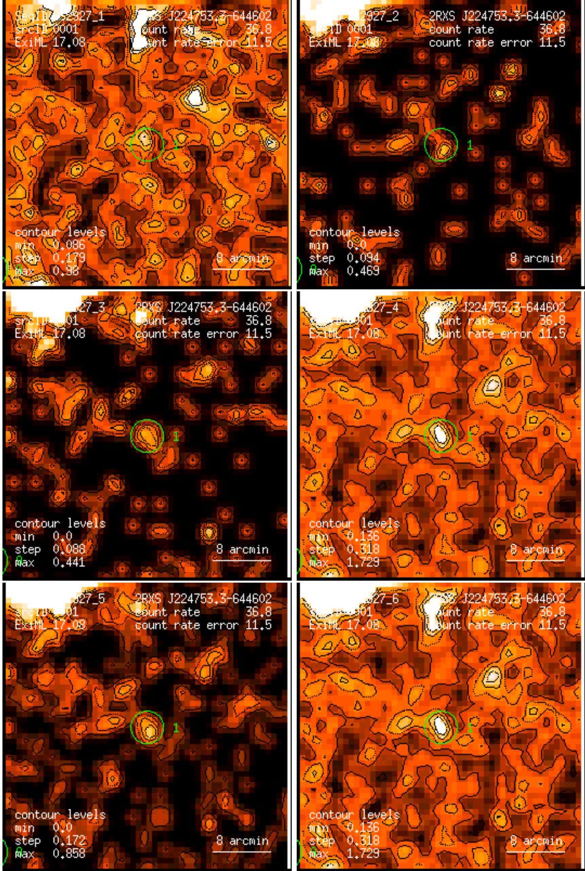
Figure 1: RASS 932927: detection 0001: band rate images, Gaussian filter: (1) PSPC channels 11 – 41, (2) 52 – 90, (3) 91 – 201, (4) 11 – 235, (5) 52 – 201, (6) 11 – 201. Broad band rates in counts/ks. Band rate contour levels in counts/ks/arcmin 2 .
