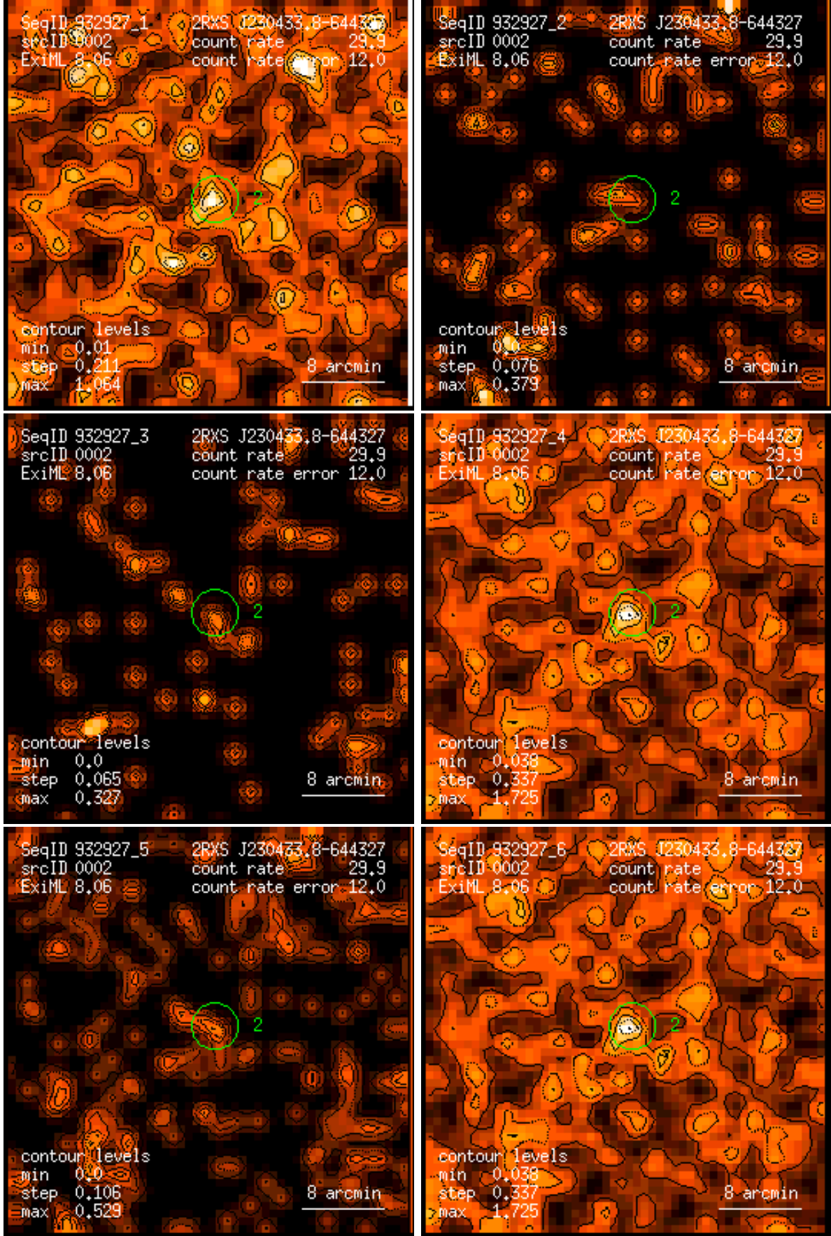
Figure 2: RASS 932927: detection 0002: band rate images, Gaussian filter: (1) PSPC channels 11 – 41, (2) 52 – 90, (3) 91 – 201, (4) 11 – 235, (5) 52 – 201, (6) 11 – 201. Broad band rates in counts/ks. Band rate contour levels in counts/ks/arcmin 2 .
