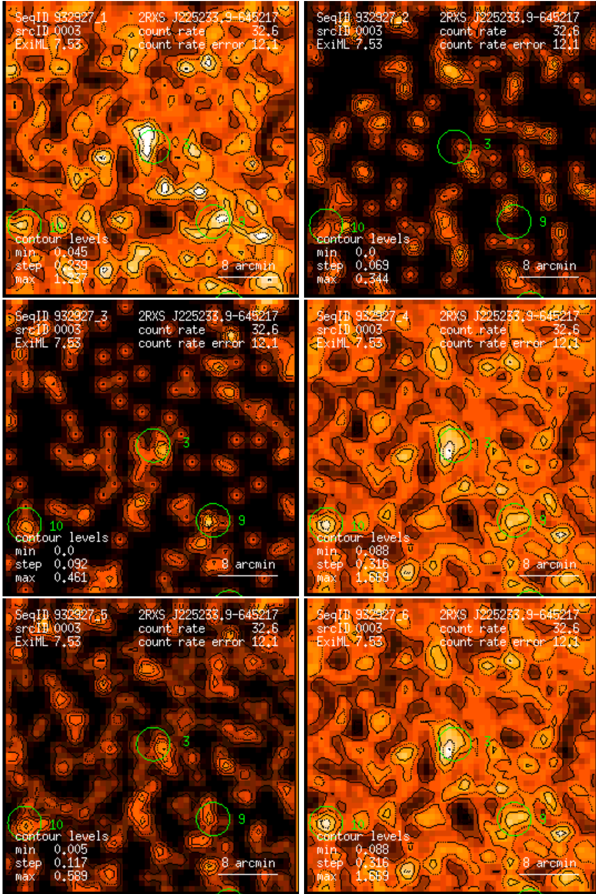
Figure 3: RASS 932927: detection 0003: band rate images, Gaussian filter: (1) PSPC channels 11 – 41, (2) 52 – 90, (3) 91 – 201, (4) 11 – 235, (5) 52 – 201, (6) 11 – 201. Broad band rates in counts/ks. Band rate contour levels in counts/ks/arcmin 2 .
