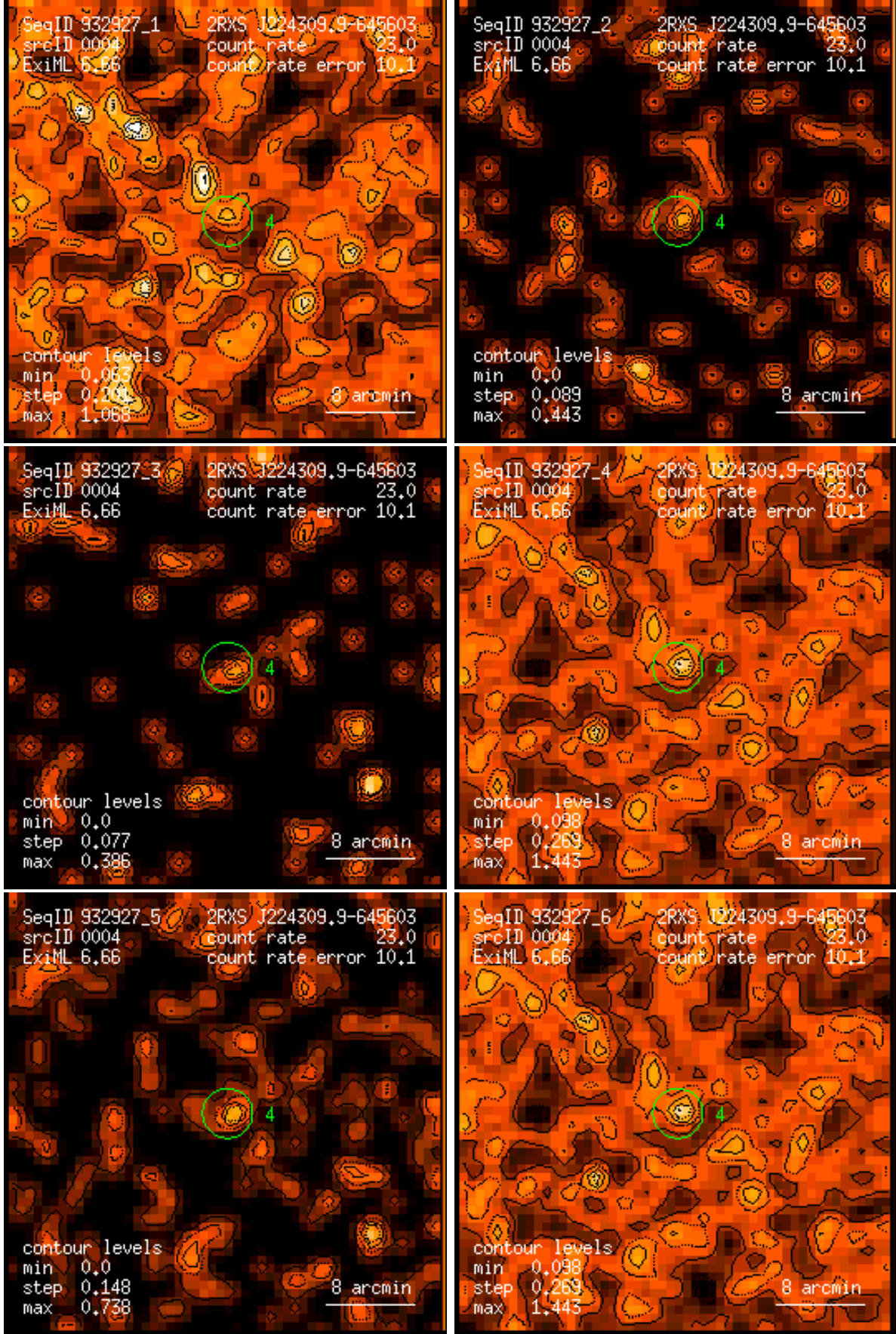
Figure 4: RASS 932927: detection 0004: band rate images, Gaussian filter: (1) PSPC channels 11 – 41, (2) 52 – 90, (3) 91 – 201, (4) 11 – 235, (5) 52 – 201, (6) 11 – 201. Broad band rates in counts/ks. Band rate contour levels in counts/ks/arcmin 2 .
