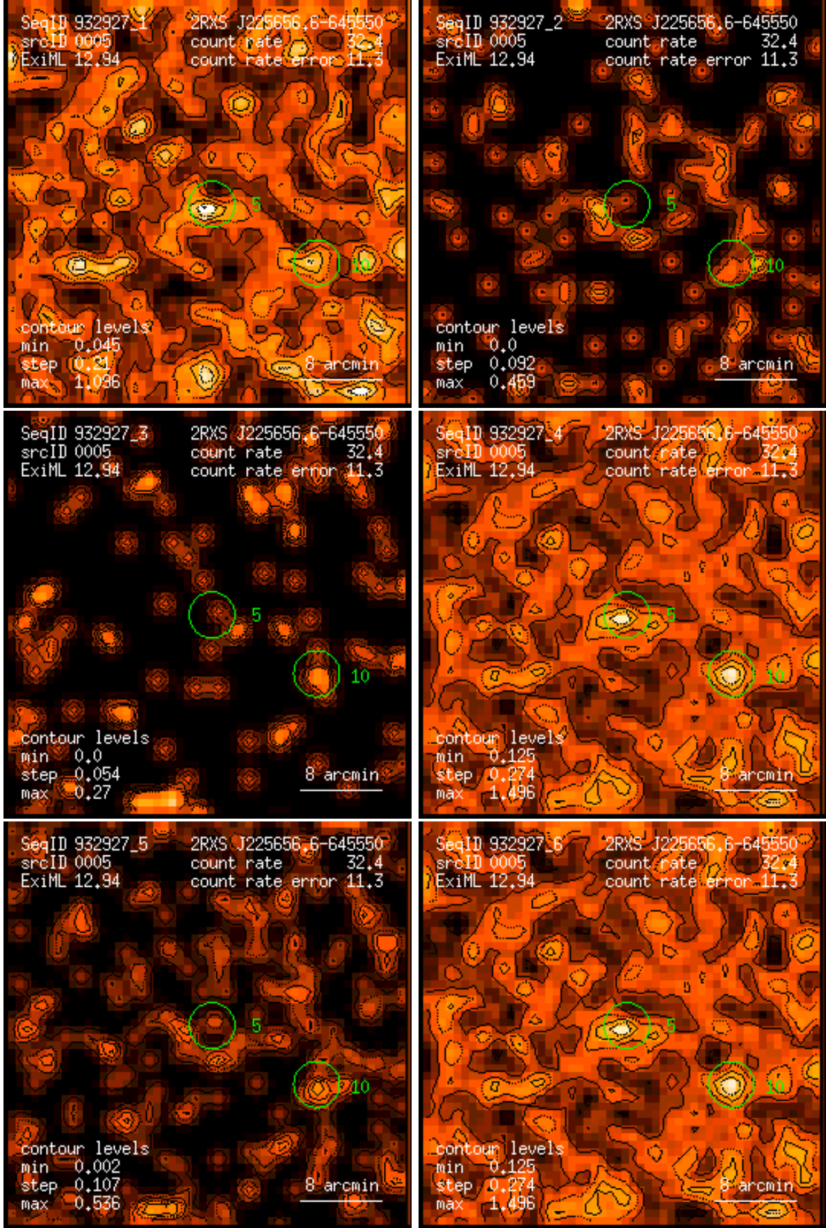
Figure 5: RASS 932927: detection 0005: band rate images, Gaussian filter: (1) PSPC channels 11 – 41, (2) 52 – 90, (3) 91 – 201, (4) 11 – 235, (5) 52 – 201, (6) 11 – 201. Broad band rates in counts/ks. Band rate contour levels in counts/ks/arcmin 2 .
