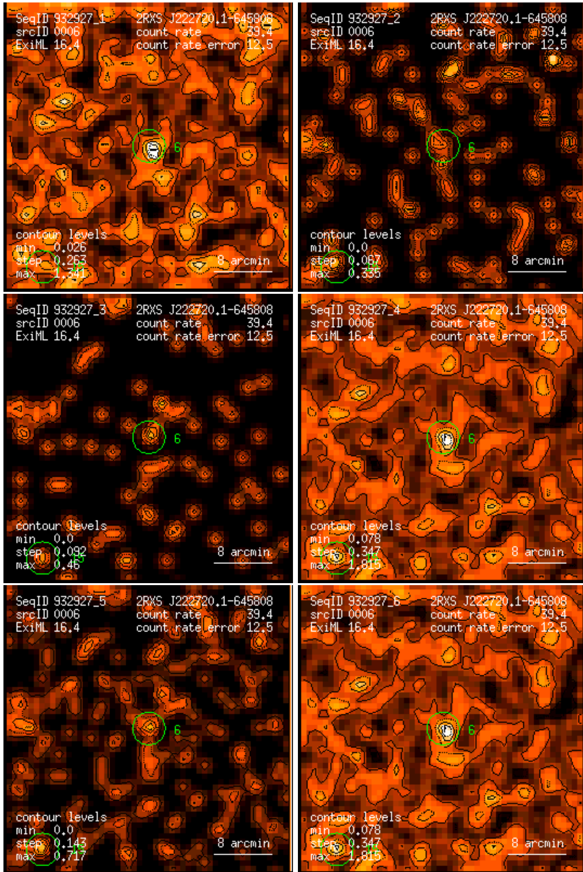
Figure 6: RASS 932927: detection 0006: band rate images, Gaussian filter: (1) PSPC channels 11 – 41, (2) 52 – 90, (3) 91 – 201, (4) 11 – 235, (5) 52 – 201, (6) 11 – 201. Broad band rates in counts/ks. Band rate contour levels in counts/ks/arcmin 2 .
