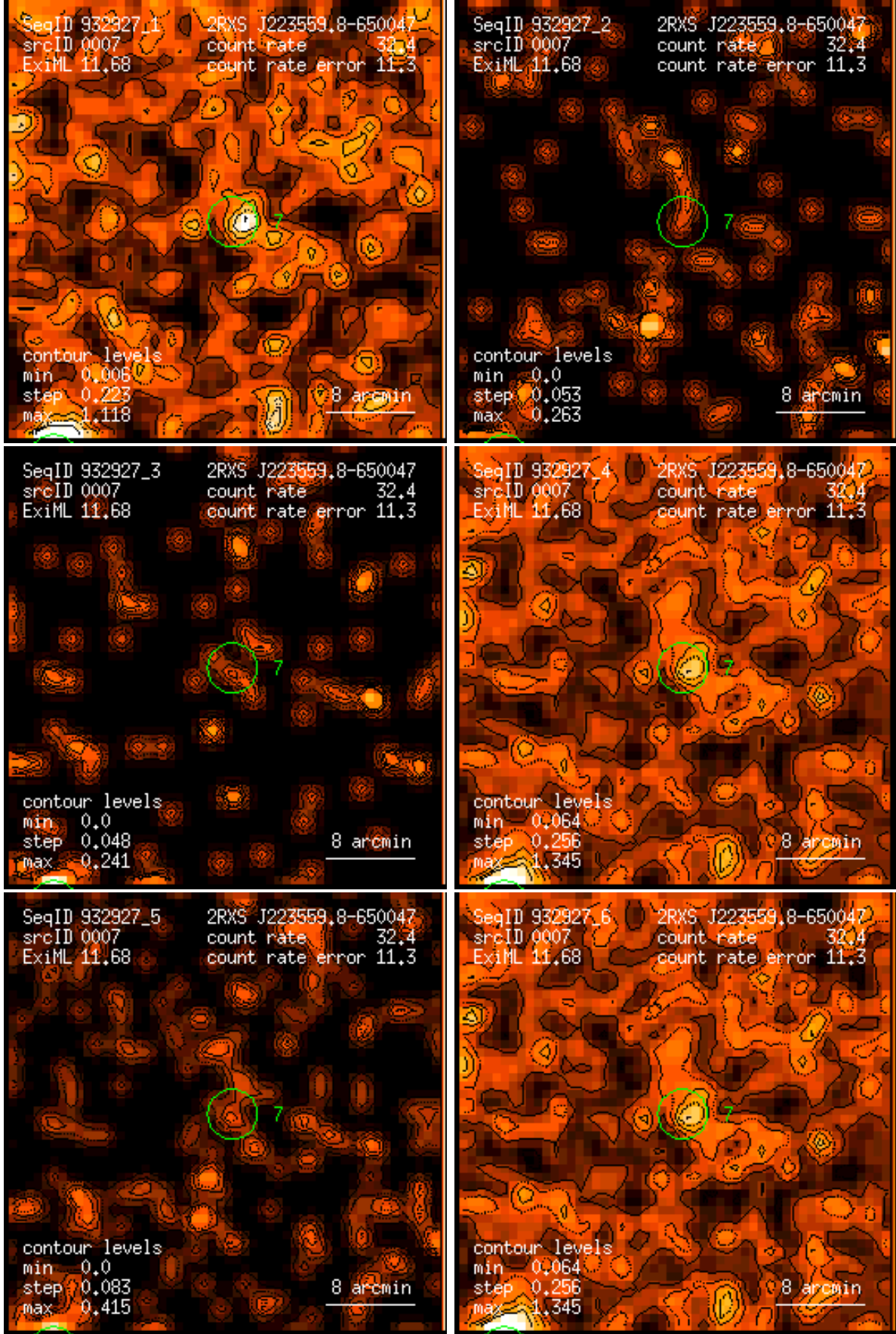
Figure 7: RASS 932927: detection 0007: band rate images, Gaussian filter: (1) PSPC channels 11 – 41, (2) 52 – 90, (3) 91 – 201, (4) 11 – 235, (5) 52 – 201, (6) 11 – 201. Broad band rates in counts/ks. Band rate contour levels in counts/ks/arcmin 2 .
