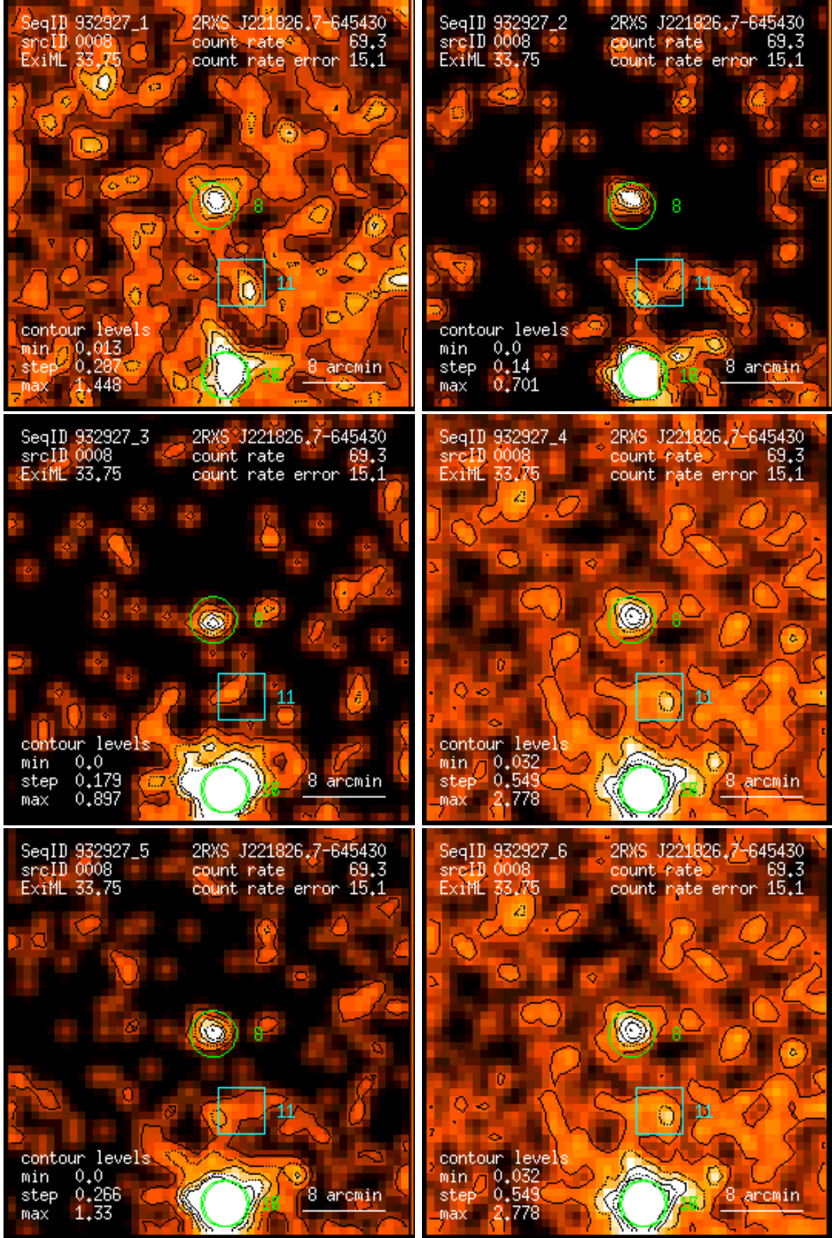
Figure 8: RASS 932927: detection 0008: band rate images, Gaussian filter: (1) PSPC channels 11 – 41, (2) 52 – 90, (3) 91 – 201, (4) 11 – 235, (5) 52 – 201, (6) 11 – 201. Broad band rates in counts/ks. Band rate contour levels in counts/ks/arcmin 2 .
