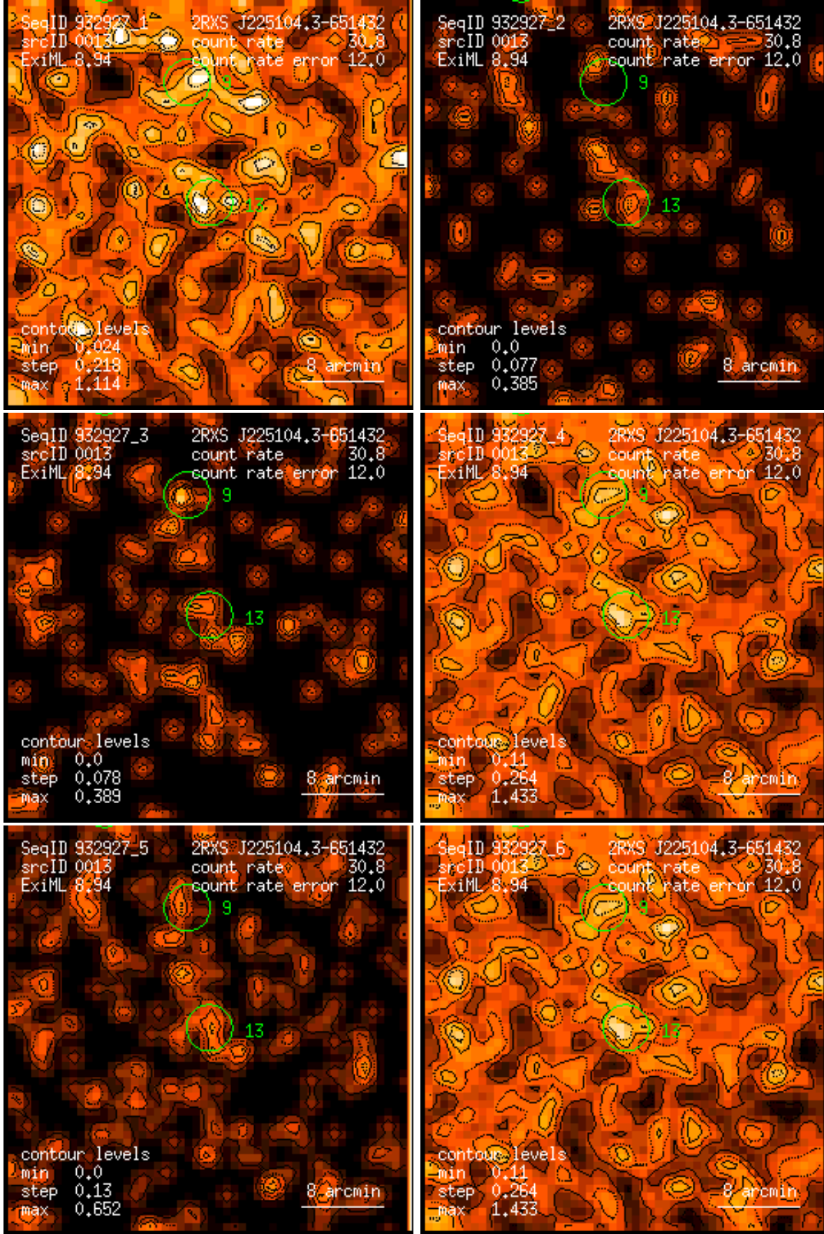
Figure 13: RASS 932927: detection 0013: band rate images, Gaussian filter: (1) PSPC channels 11 – 41, (2) 52 – 90, (3) 91 – 201, (4) 11 – 235, (5) 52 – 201, (6) 11 – 201. Broad band rates in counts/ks. Band rate contour levels in counts/ks/arcmin 2 .
