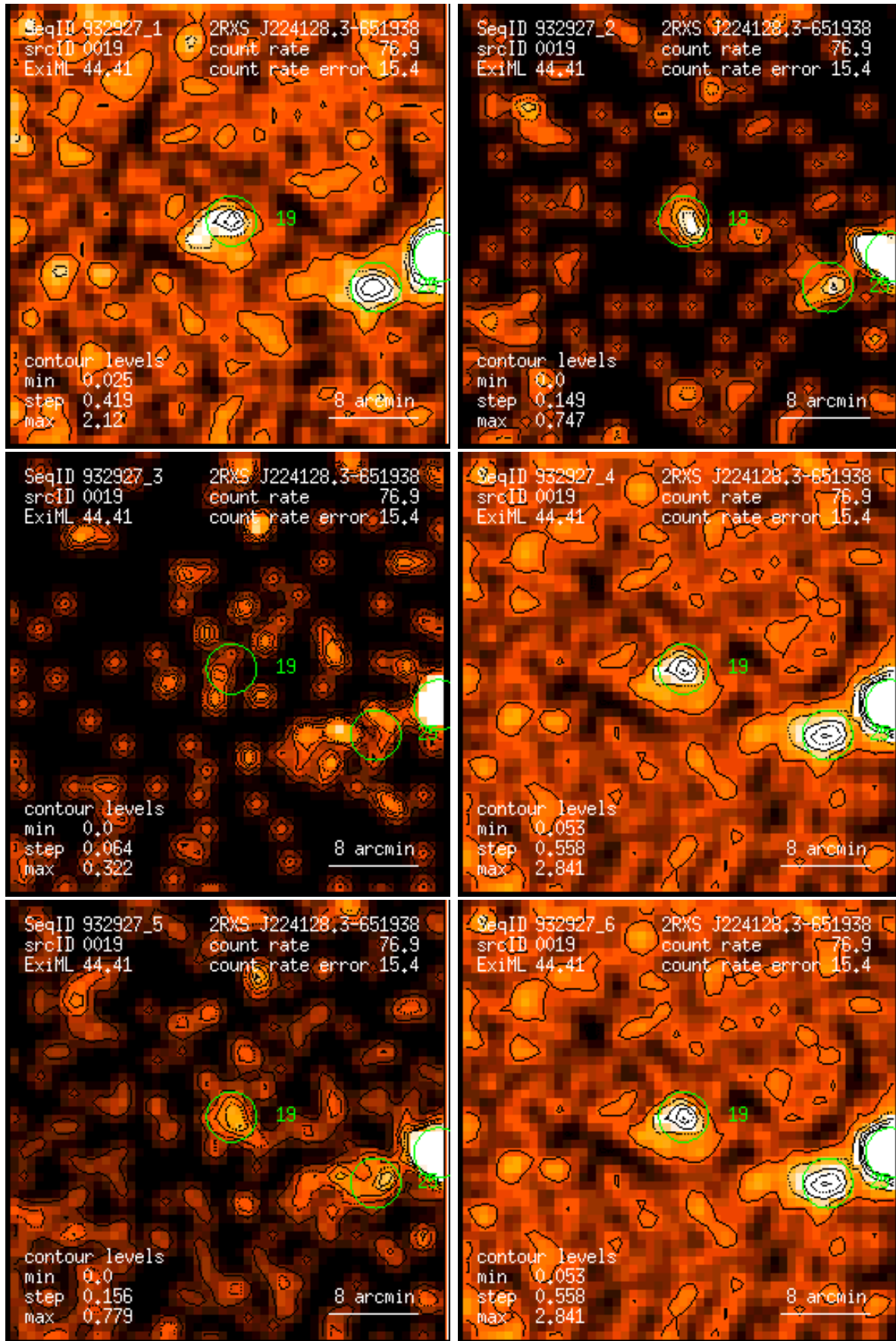
Figure 19: RASS 932927: detection 0019: band rate images, Gaussian filter: (1) PSPC channels 11 – 41, (2) 52 – 90, (3) 91 – 201, (4) 11 – 235, (5) 52 – 201, (6) 11 – 201. Broad band rates in counts/ks. Band rate contour levels in counts/ks/arcmin 2 .
