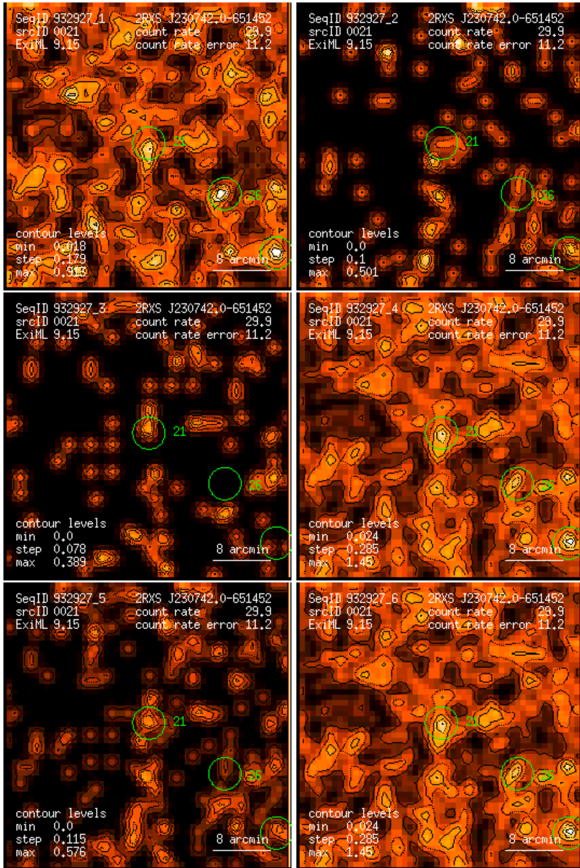
Figure 21: RASS 932927: detection 0021: band rate images, Gaussian filter: (1) PSPC channels 11 – 41, (2) 52 – 90, (3) 91 – 201, (4) 11 – 235, (5) 52 – 201, (6) 11 – 201. Broad band rates in counts/ks. Band rate contour levels in counts/ks/arcmin 2 .
