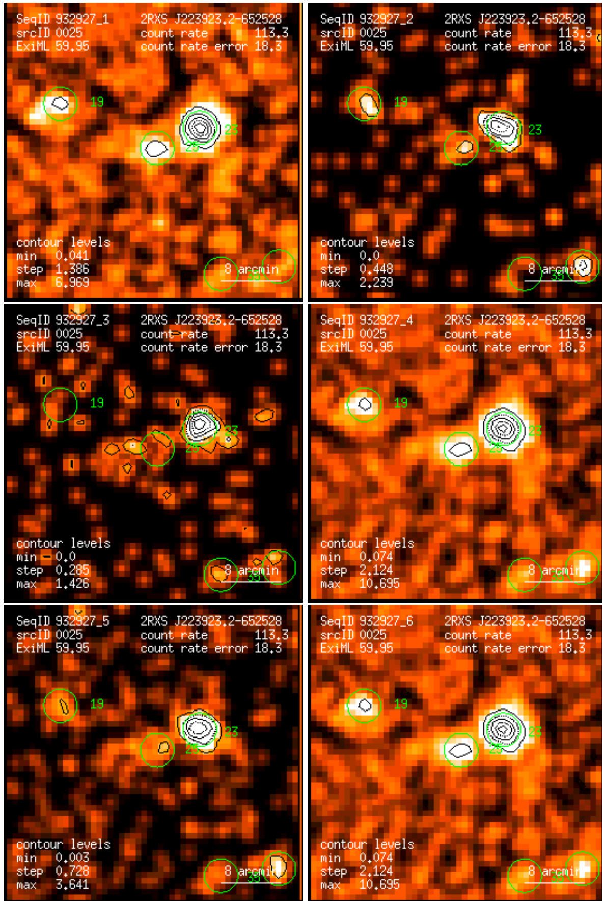
Figure 25: RASS 932927: detection 0025: band rate images, Gaussian filter: (1) PSPC channels 11 – 41, (2) 52 – 90, (3) 91 – 201, (4) 11 – 235, (5) 52 – 201, (6) 11 – 201. Broad band rates in counts/ks. Band rate contour levels in counts/ks/arcmin 2 .
